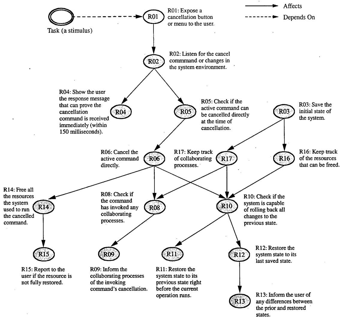
Figure 7: Responsibility Graph After Adding Application-Level Cancellation Responsibilities
