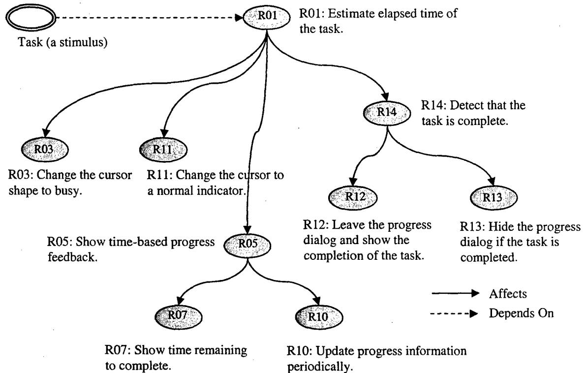
Figure 5: Responsibility Graph After Adding Time-Based Progress Feedback Responsibilities
