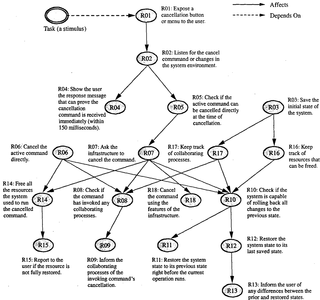
Figure 8: Responsibility Graph After Adding Infrastructure-Level Cancellation Responsibilities
