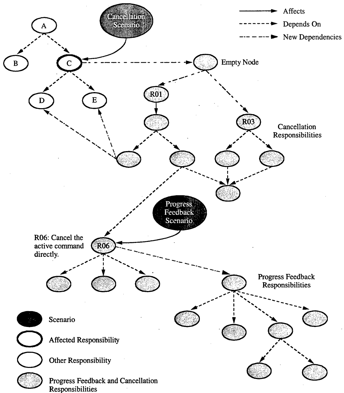
Figure 9: Responsibility Graph After Adding Progress Feedback Responsibilities
