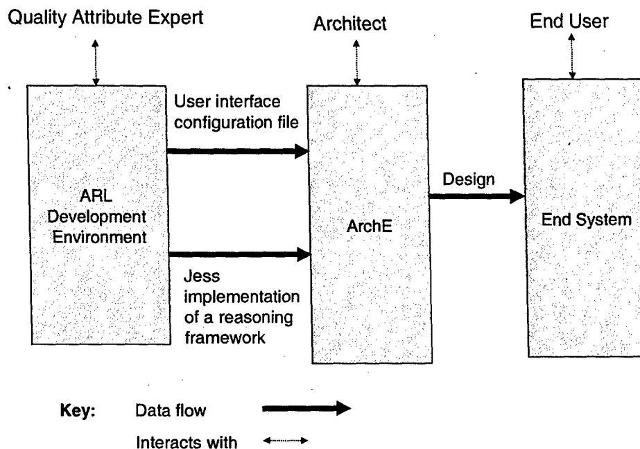
Figure 1: Information Flow from the Specification of a Reasoning Framework to an End User
