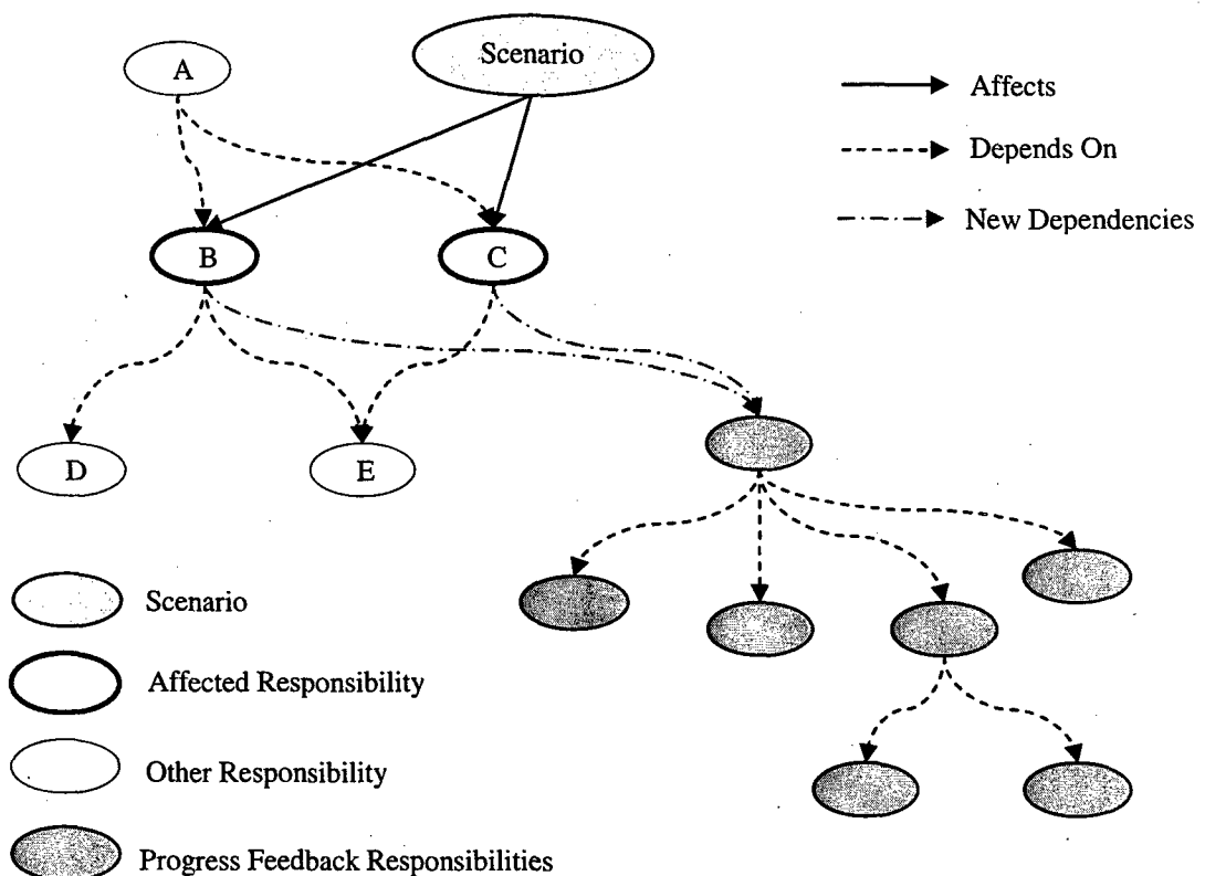
Figure 3: Responsibility Graph Linked to Scenario Before the Actions of the Reasoning Framework
