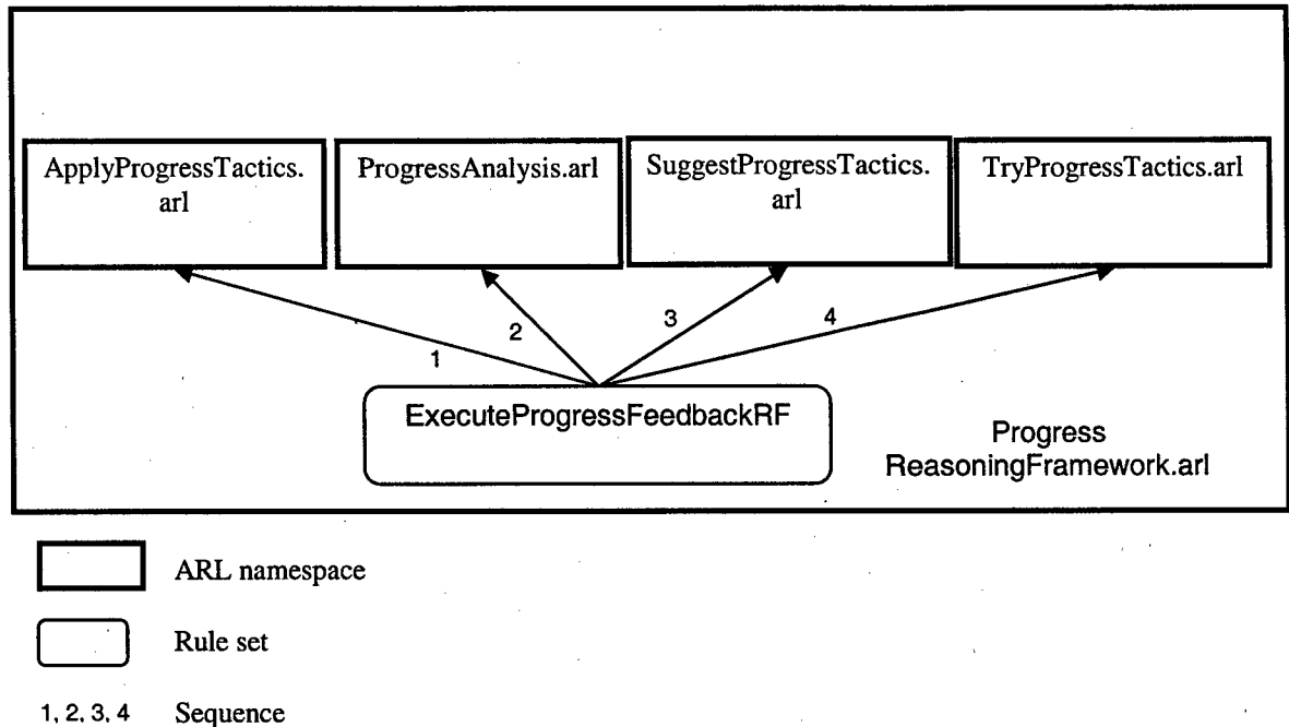
Figure 10: ARL Namespaces for Progress Feedback
