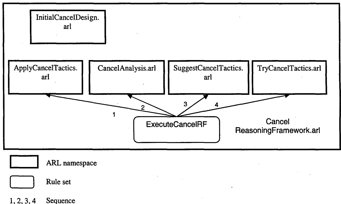
Figure 11: ARL Namespaces for Cancellation
