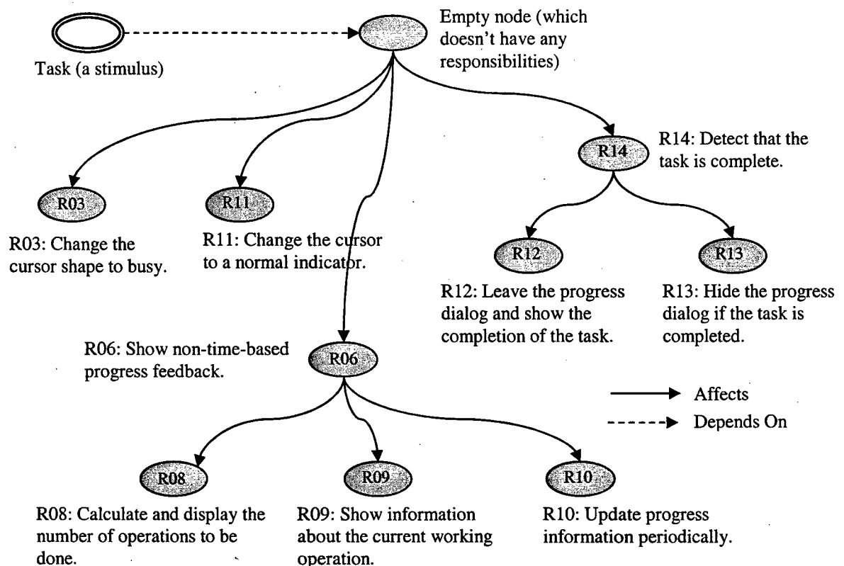
Figure 6: Responsibility Graph After Adding Non-Time-Based Progress Feedback Responsibilities
