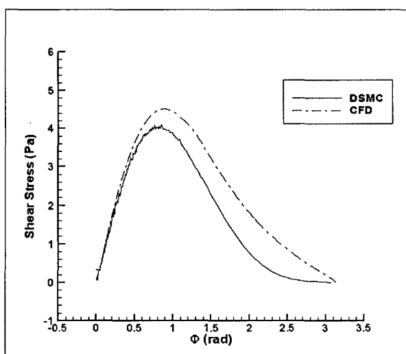
Figure 19. Kn = 0.05 surface shear stress.
