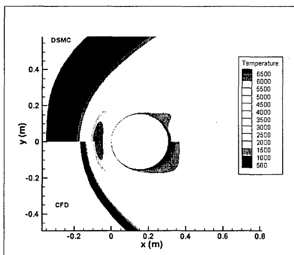
Figure 16. Kn = 0.05 temperature field.
