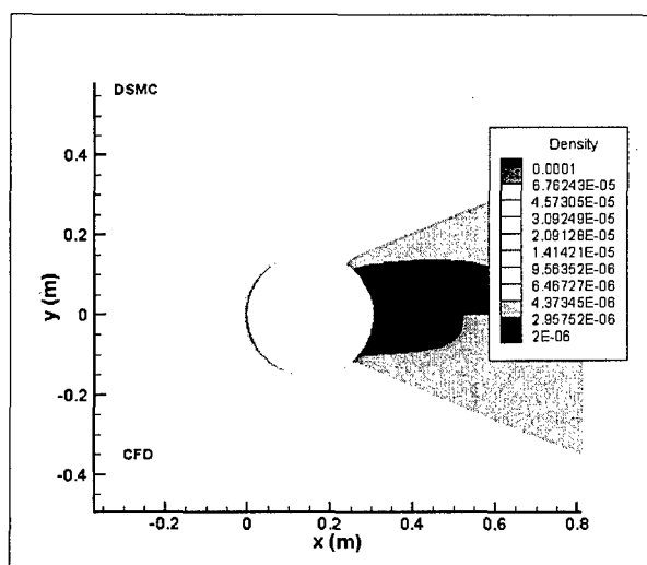
Figure 17. Kn = 0.05 density field.
