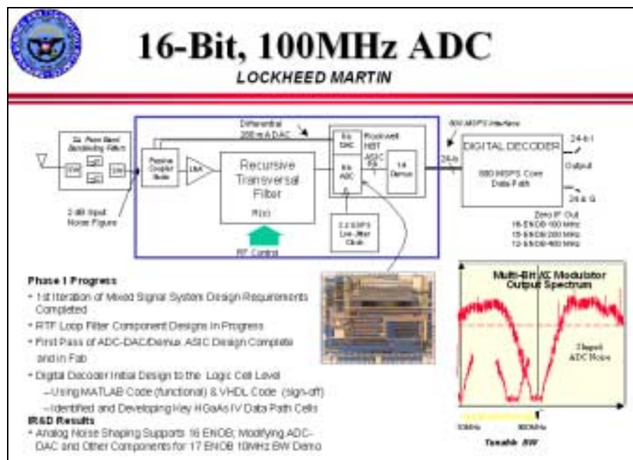
Figure 16. Lockheed Martin 16-bit, 100 MHz ADC Design
