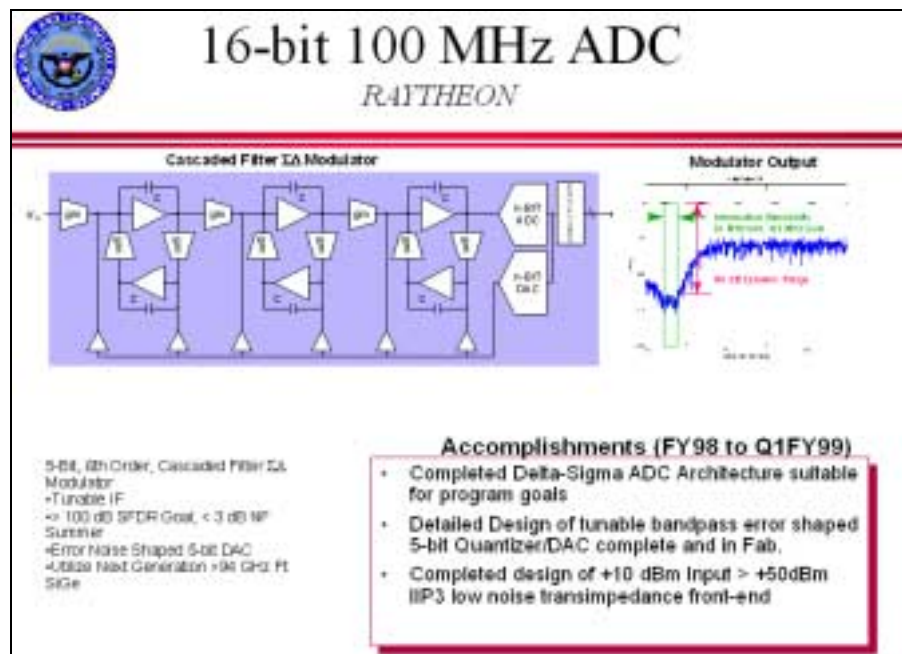
Figure 15. Raytheon 16-bit, 100 MHz ADC Design
