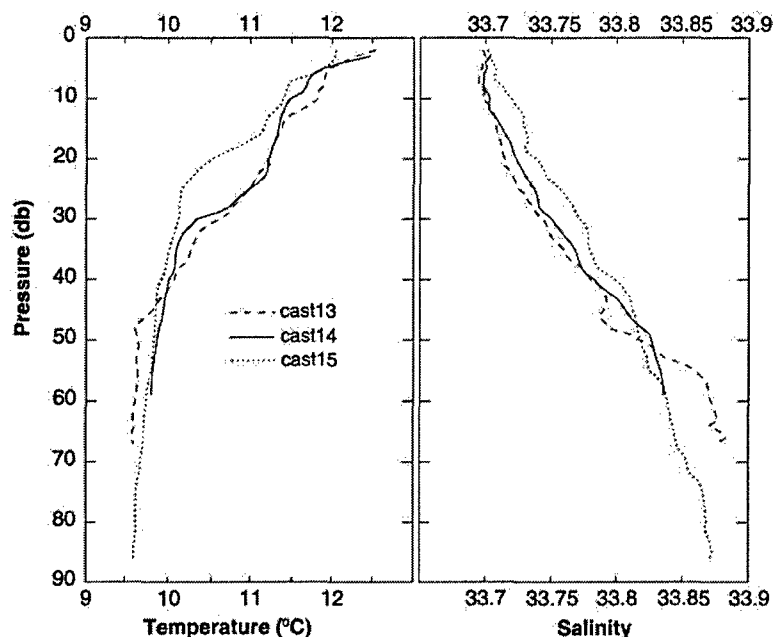
Figure 7. A time series of CTD profiles collected from the R/V New Horizon on 23 August 2000. All were collected very near 36.87°N, 122.00°W. The dashed, solid, and dotted lines were collected at 0100, 1000, and 1130 LT, respectively.
