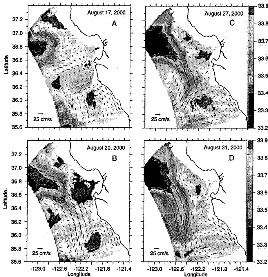
Figure 15. Salinity and current vectors at 100 m depth for the entire ICON model domain, for (a) 17 August, (b) 20 August, (c) 27 August, and (d) 31 August 2000.
