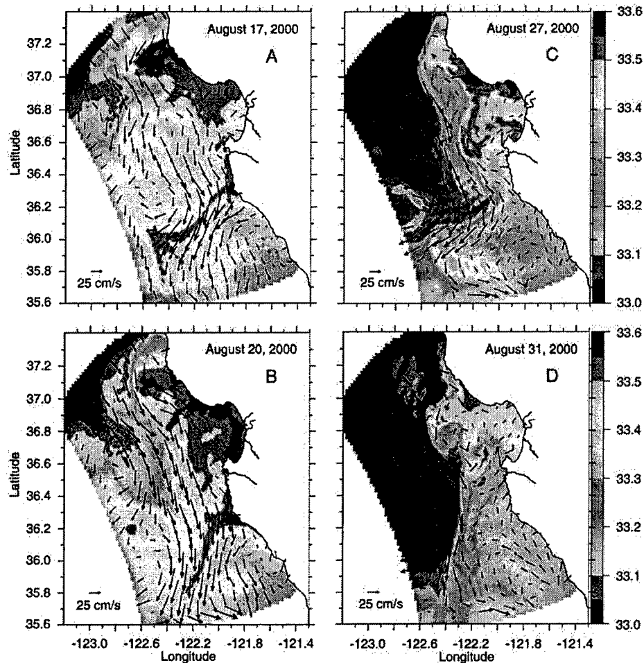
Figure 14. Surface salinity and velocity vectors for the entire ICON model domain from (a) 17 August, (b) 20 August, (c) 27 August, and (d) 31 August 2000.
