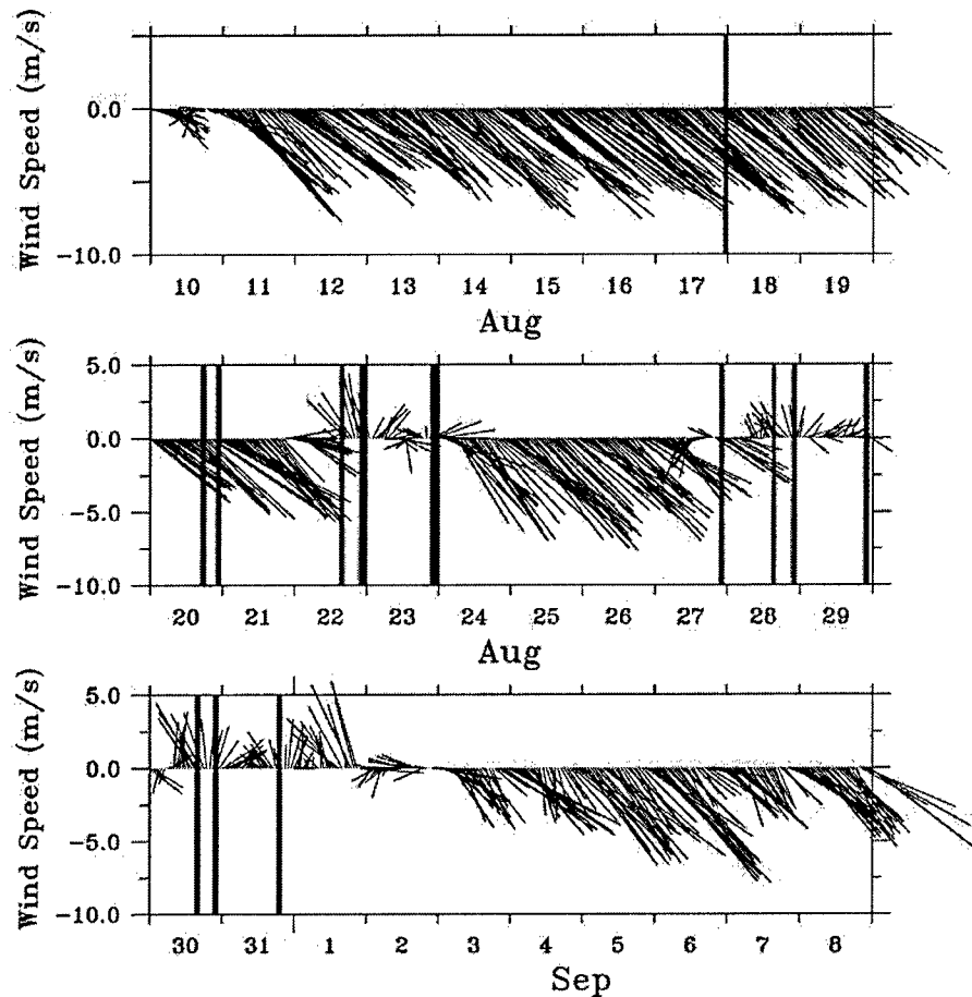
Figure 3. Wind speed and direction from 10 August to 8 September from NOAA buoy 46042 located just off the mouth of the Monterey Bay (see location in Figure 1). The length of the lines indicates the wind speed and the orientation indicates the direction the wind is blowing toward (oceanographic convention). The shaded lines indicate the times when the aircraft overflights were performed.
