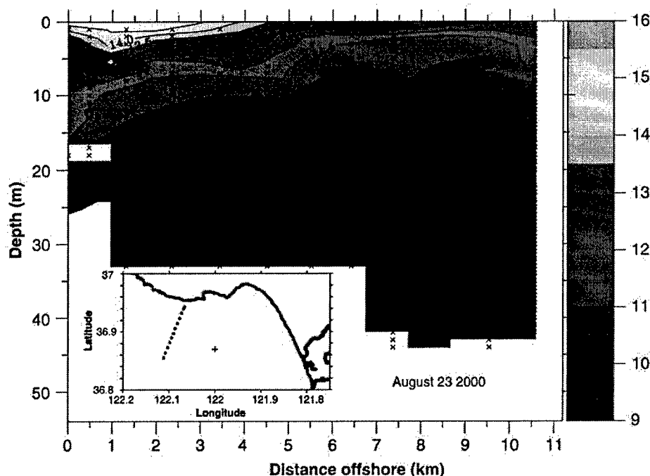
Figure 6. Temperature transect off Santa Cruz, California, collected from the R/V Ricketts during the early morning hours of 23 August 2000. Note the very shallow stratified layer that existed in the upper 5 m of the water column. The inset shows the transect location in the northern part of the Monterey Bay. The cross indicates the location of the CTD profiles shown in Figure 7.
