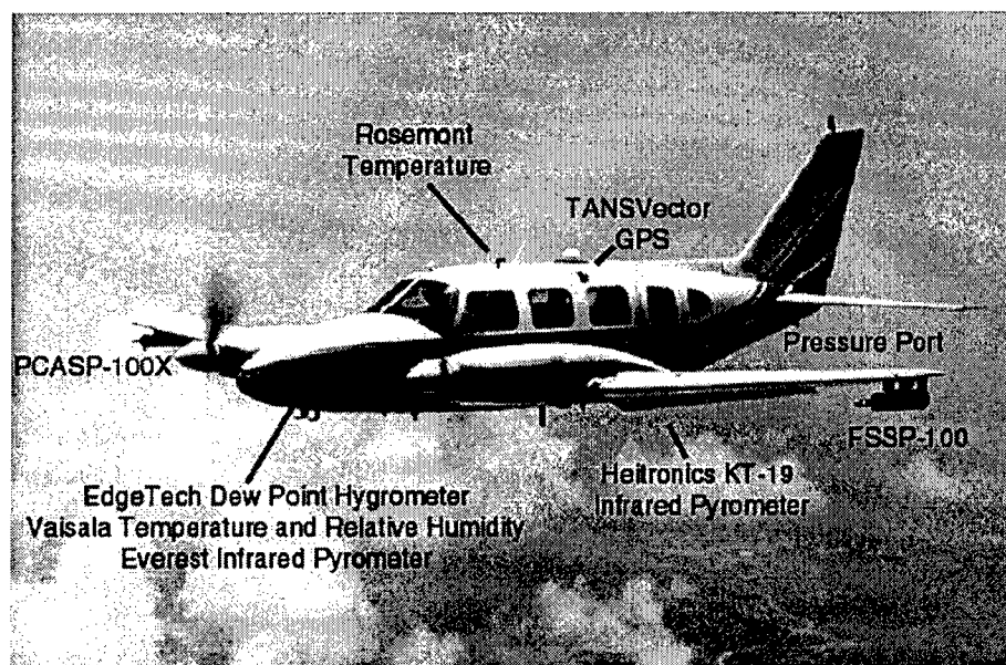
Figure 2. The Navajo aircraft with the positions of the various on-board sensors noted.
