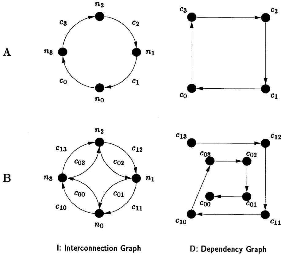
Figure 2: Breaking Deadlock with Virtual Channels
