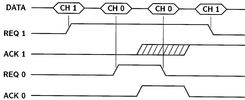
Figure 8: Channel Protocol Example
