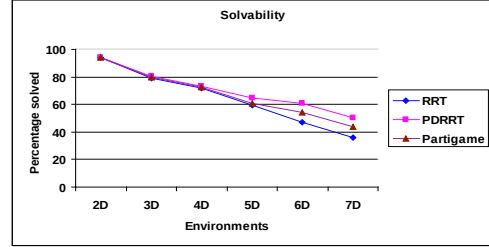
Fig. 7. Number of motion-planning problems solved in random terrain
