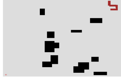
Fig. 6. Randomly generated terrain with a four-link robot at the start location (upper-right corner) and a small square at the goal location (lower-left corner)
