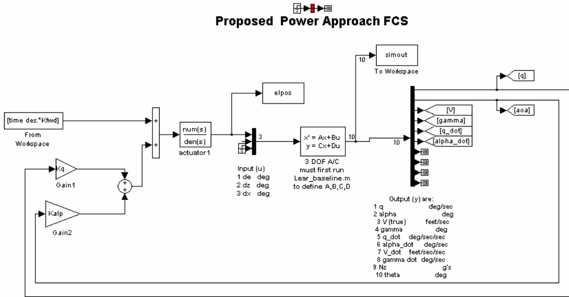
Figure 19. Updated Closed Loop Simulink Model
