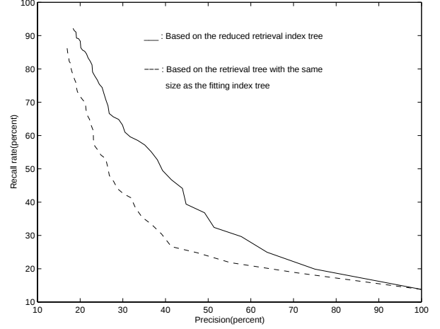
Figure 5: Precision versus recall for population-based retrieval.
