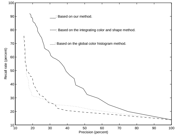
Figure 6: Comparison of precision versus recall rate.
