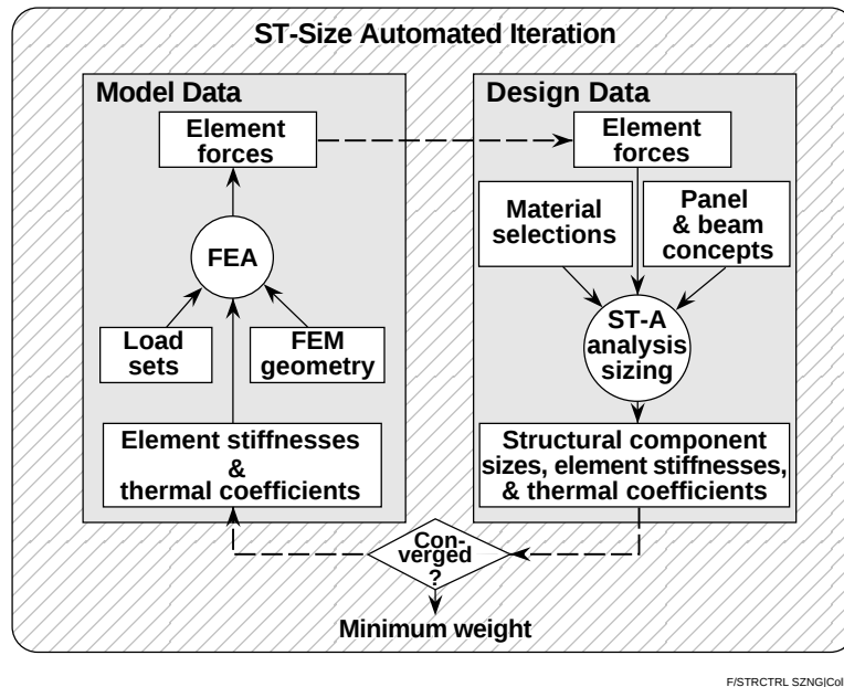
Figure 2 The HyperSizer structural sizing process.
