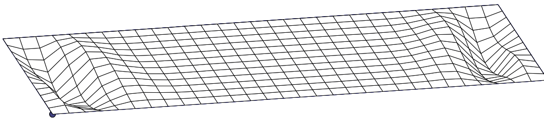
Figure 15 Lowest buckling mode for a corrugated stiffened container sidewall upon uniform floor loading. Note that the buckles are located at the side wall ends where the in-plane shear force is higher.
