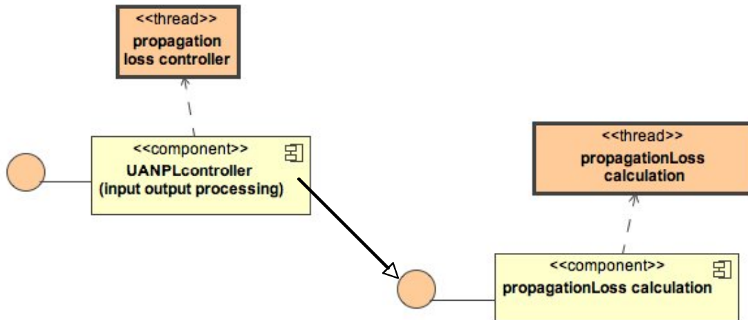
Figure 29. Implementation Diagram.
