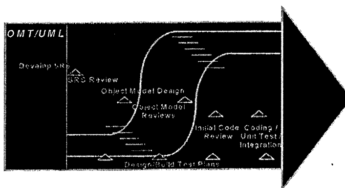
Figure 12: OMT/UML Process
