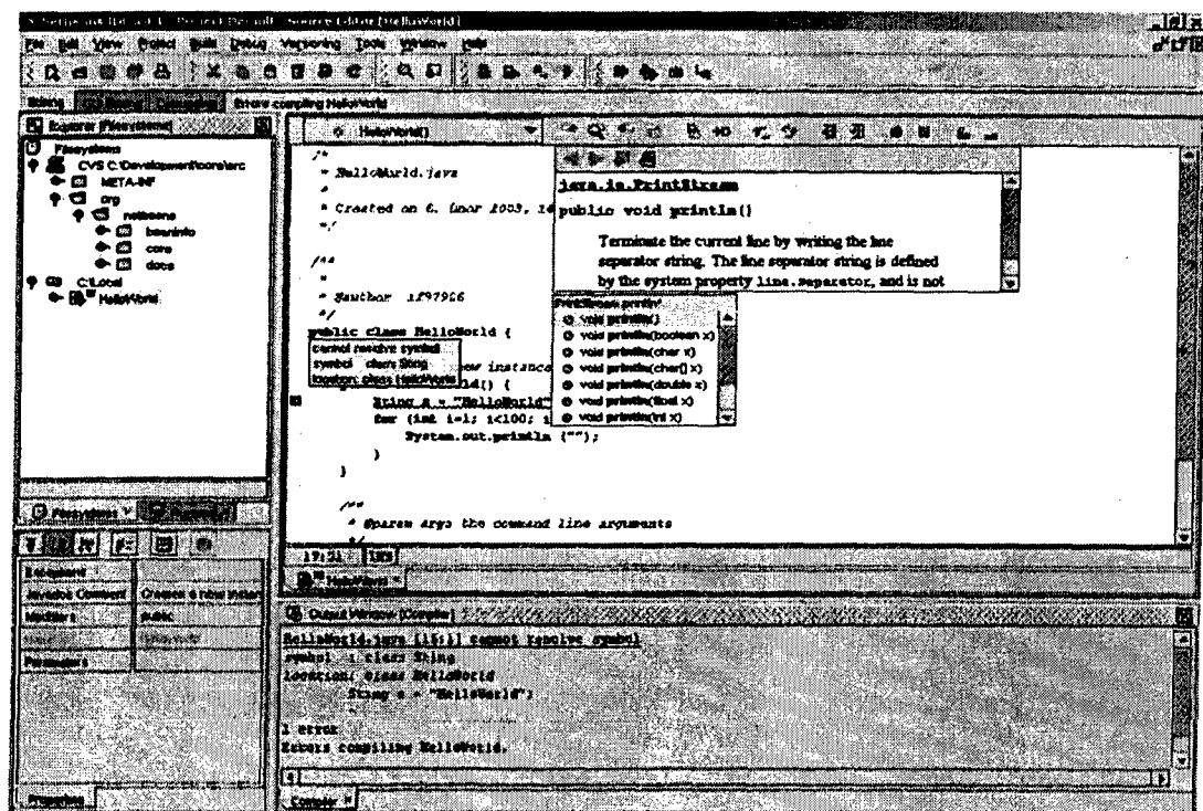
Figure 3: NetBeans IDE
