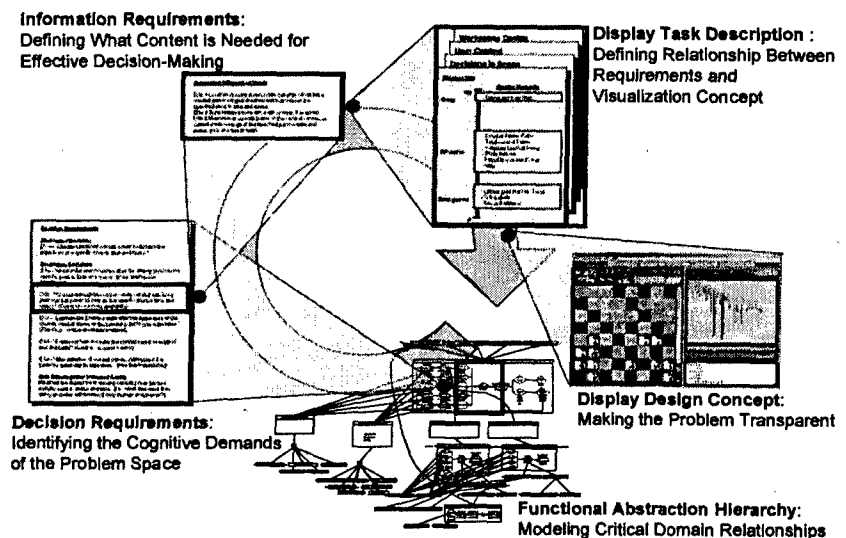
Figure 10: CSE Process
