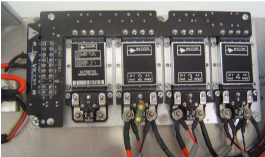
Figure 22. Vicor DC-DC Converter array
