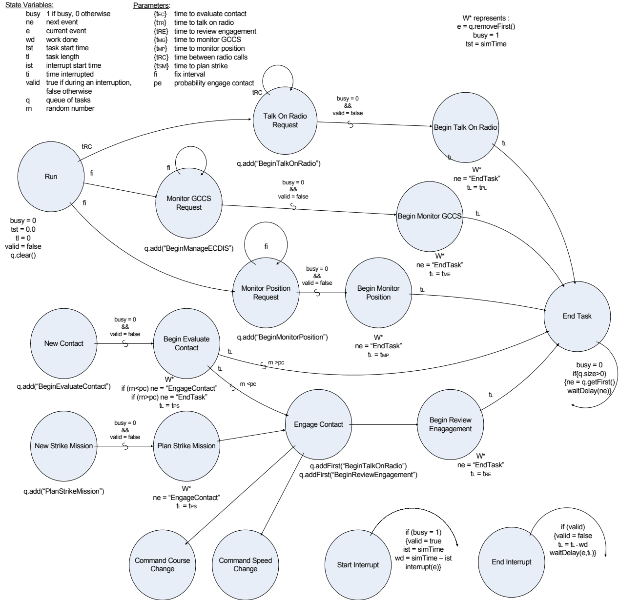
Figure 28. Tactical Action Officer Event Graph
