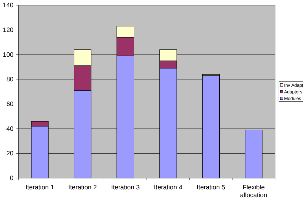
Figure 13: Adaptors vs. Modules
