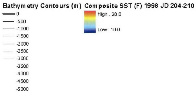
Figure 48. NEUS Composite Sea Surface Temperature for 1998, Julian Days 204-210
