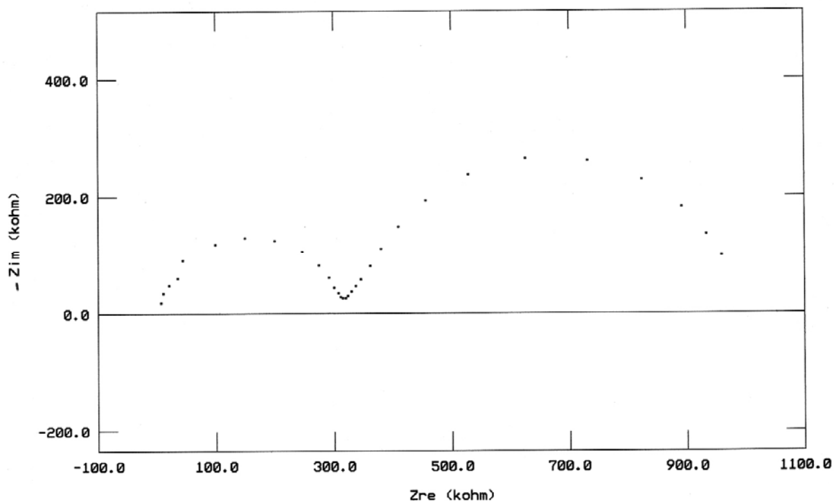
Figure 9. Nyquist plot for a pressed pellet of Li 2 Pc recrystallized from acetone and toluene and dried at 160°C under vacuum.
