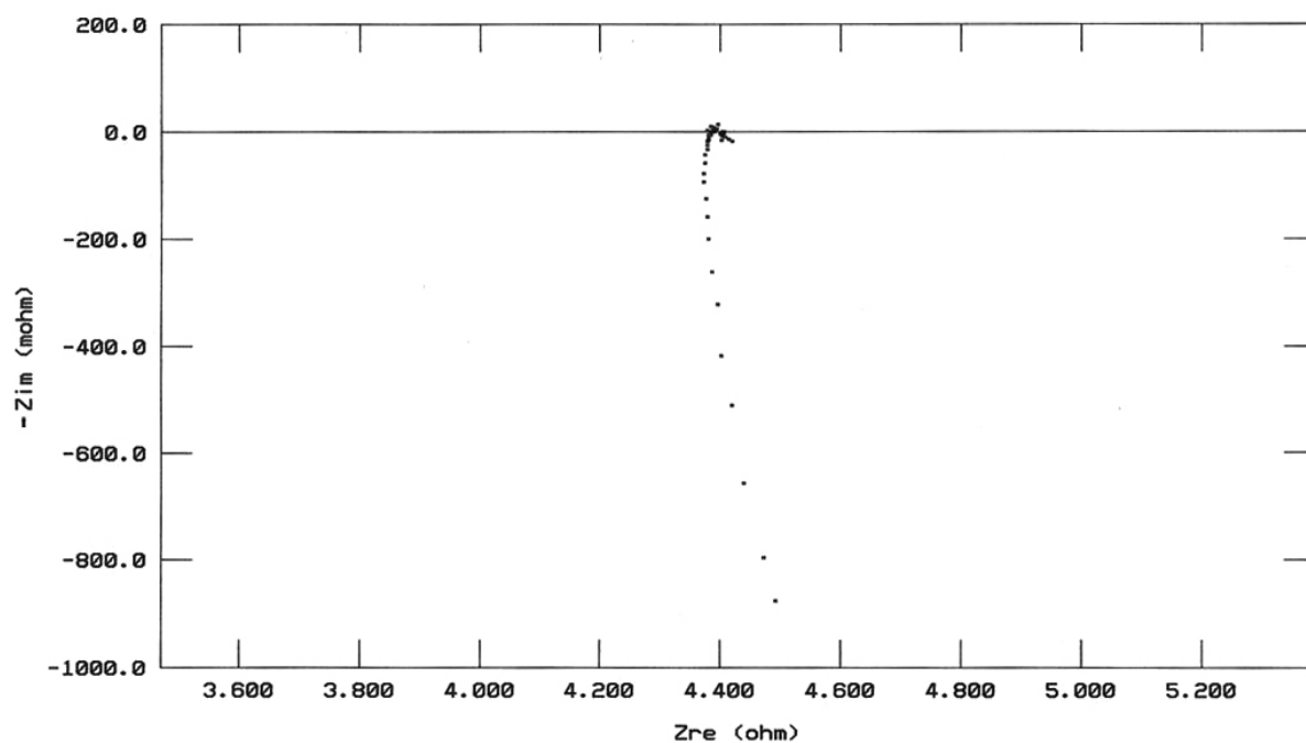
Figure 10. Nyquist plot of Cu/Li 2 Pc(Sol. Cast 20µm film4)/Au cell at 21°C and 4,000 psi.
