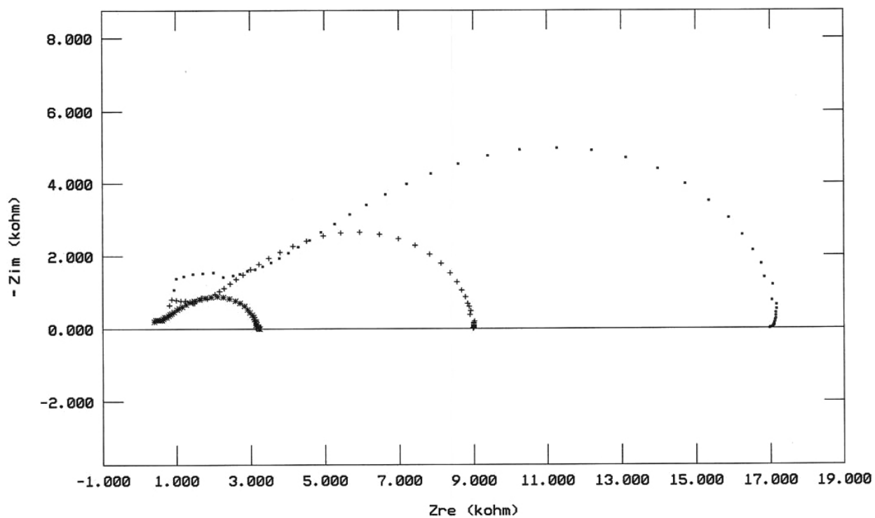
Figure 7. Nyquist plots of Cu/Li 2 Pc(Sol. Cast 20μm film 4)/Cu cell at 21°C and pressures of 24,000 psi, 12,000 psi and 8,000 psi.
