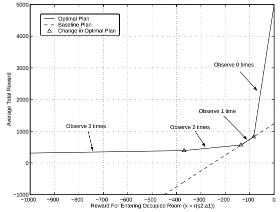
Figure 5: Average Total Rewards vs. Reward for Entering an Occupied Room ( x ) (Analytical)
