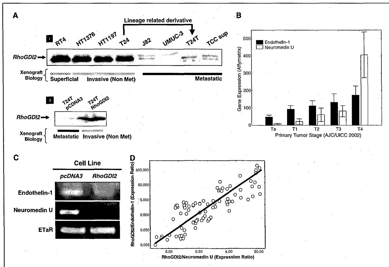
Figure 1. A, expression of RhoGDI2 protein in human bladder cell lines as a function of clinical and xenograft behavior. i , cell lysates of bladder cancer cell lines were prepared and Westerns probed with anti-RhoGDI2 antibody carried out as described (4). Xenograft behavior is indicated using color-coded lines. ii , protein expression of T24T cells stably transfected and expressing RhoGDI2 transgene or vector control (pcDNA3). B, ET-1 and NmU mRNA expression as a function of human bladder cancer stage. A set of 23 primary carcinomas (five Ta, five T1, six T2, three T3, and four T4) was macrodissected and areas comprised of >80% viable carcinoma was used for expression profiling using the Affymetrix HG-U133A array as described. Columns, mean Affymetrix expression levels as a function of stage; bars, SD. Both Et-1 ( P = 0.004 ) and NmU ( P = 0.001 ), which show significant increases in expression levels across stage, assuming a linear trend in the \ln(\text{expression level}) . C, expression of ET-1, NmU, and endothelin receptor A (ETaR) in RhoGDI2- and vector-transfected cells. RT-PCR was done with primers specific for NmU and ET-1 as described in Materials and Methods. The template used was RNA isolated from T24T-RhoGDI2 and T24T-pcDNA3 cells. D, expression ET-1 and NmU as a function of RhoGDI2 in bladder cancer cell lines. Forty-one human bladder cell lines were analyzed on oligonucleotide arrays for the expression levels of RhoGDI2, NmU, and ET-1. Ratio of NmU to RhoGDI2 expression (X-axis); ratio of endothelin to RhoGDI2 expression (Y-axis). Regression line is shown. Correlation = 0.85; 95% confidence interval, 0.78-0.90; P < 0.001 .
