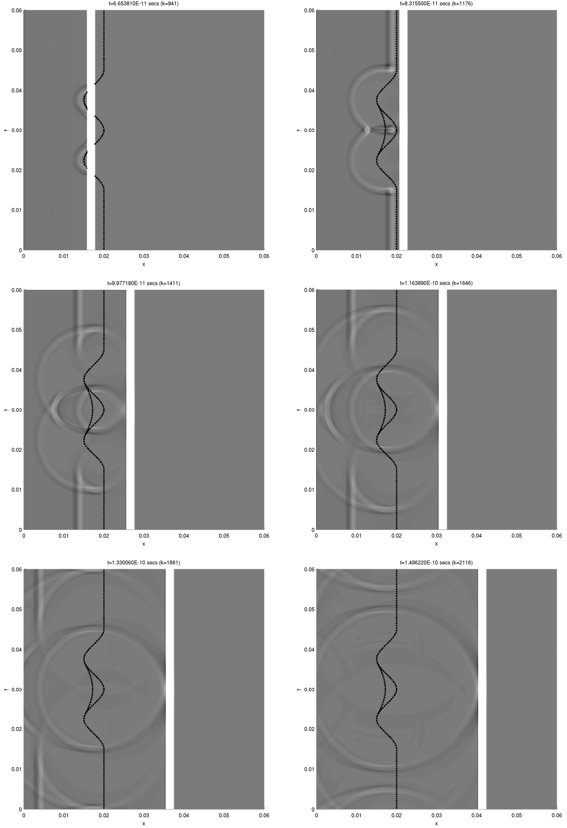
Figure 3: Surface plots of solutions for the case where the indices of refraction n_1 and n_2 are used in the low density part of the foam and in the knit lines, respectively (i.e., the presence of knit lines is not ignored).
