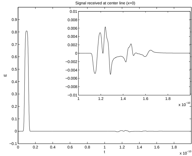
Figure 5: : Signal received at x = 0 on the center line for the case where the knit lines and surrounding regions are modeled separately (the inset is a magnification of the reflection).
