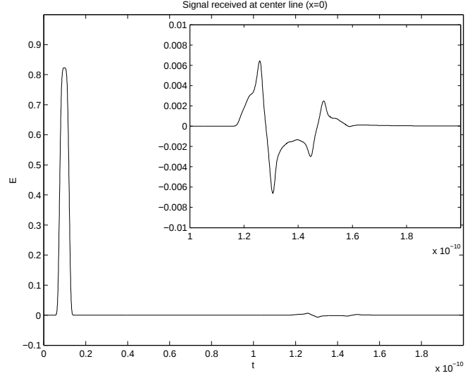
Figure 4: Signal received at x = 0 on the center line for the homogeneous case (the inset is a magnification of the reflection).
