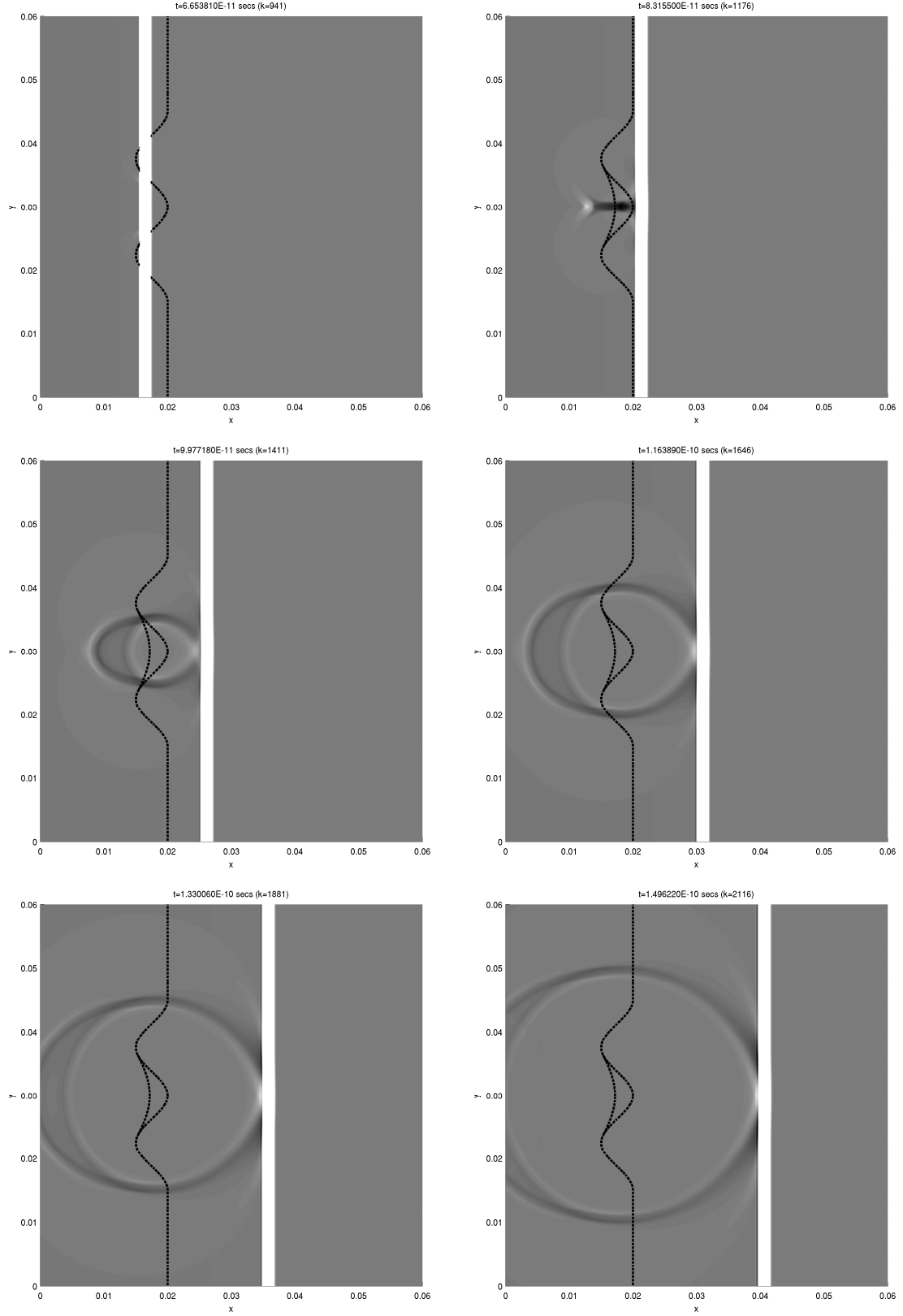
Figure 2: Surface plots of solutions for the case where the effective index of refraction is used in the low density part of the foam and in the knit lines (i.e., the presence of knit lines is ignored).
