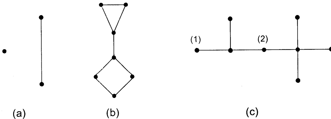
(U) Figure 1: Examples of graphs
