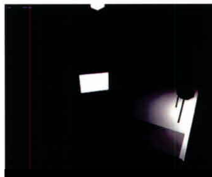
Figure 6 - Local Illumination
