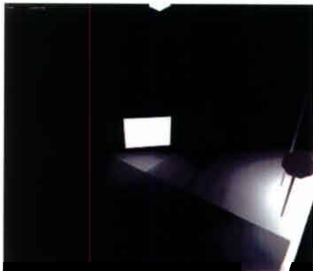
Figure 7 - Global Illumination
