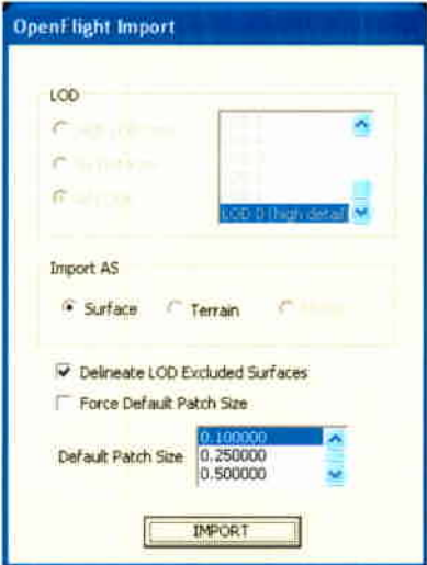
Figure 15 - Import Dialog
