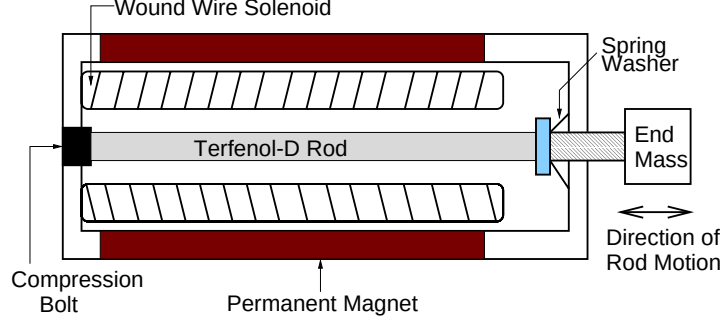
Figure 1. Terfenol-D transducer.
