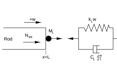
Figure 6. Rod model.
