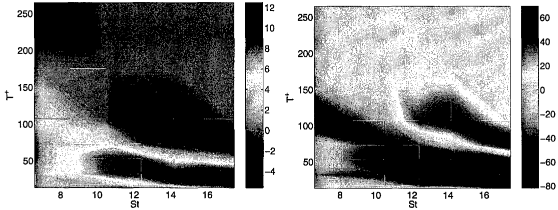
Figure 3.6: Percent change in flow rate and production terms over a wide range of forcing frequencies and amplitudes for a flow rate of Re^* = 167 . The maximum increase in flow rate is accompanied by the greatest decrease in turbulence production, near the 'sweet spot'.
