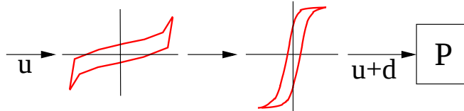
Figure 3: Approximate model inverse employed as a filter for robust control design in hysteretic and nonlinear systems.
