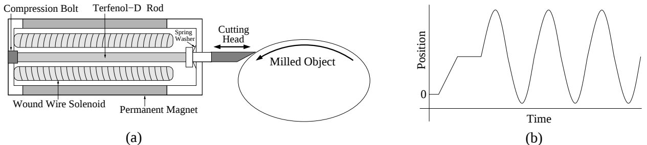
Figure 1: (a) Prototypical magnetostriuctive transducer used for high speed, high accuracy milling. (b) Trajectory to be tracked by the cutting head.
