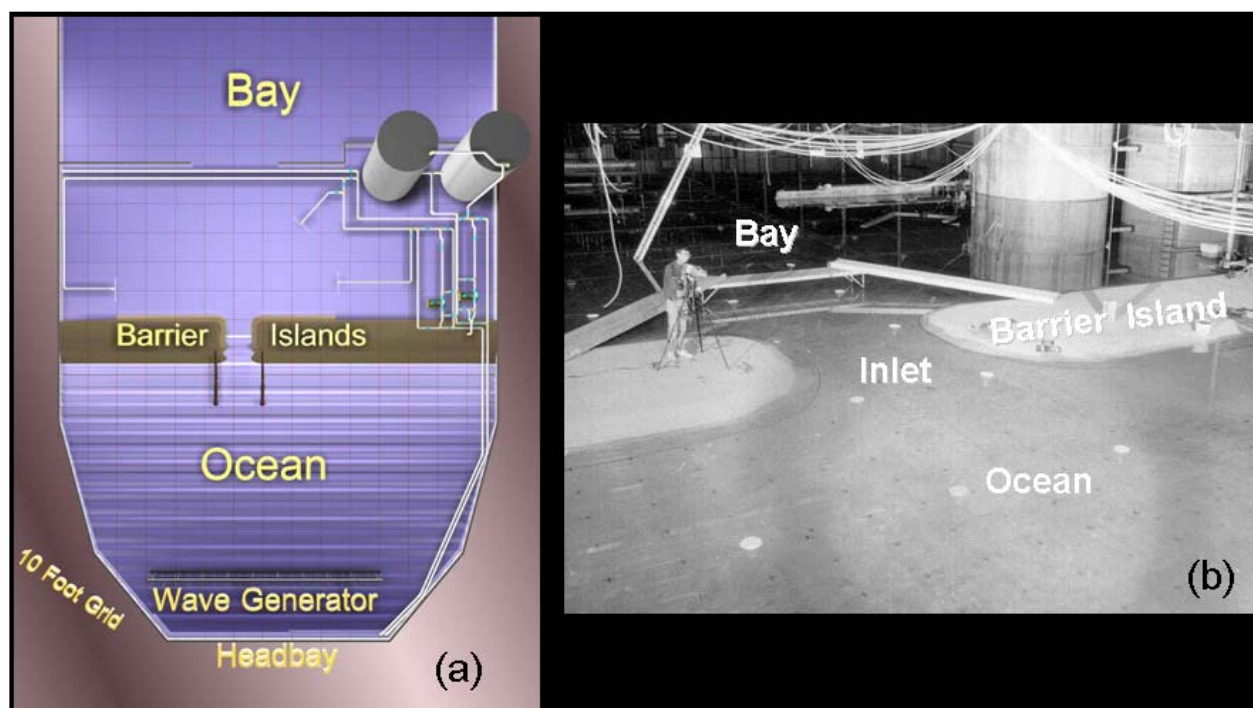
Figure 2. CIRP idealized inlet (a) physical model layout and (b) photograph of idealized inlet model
