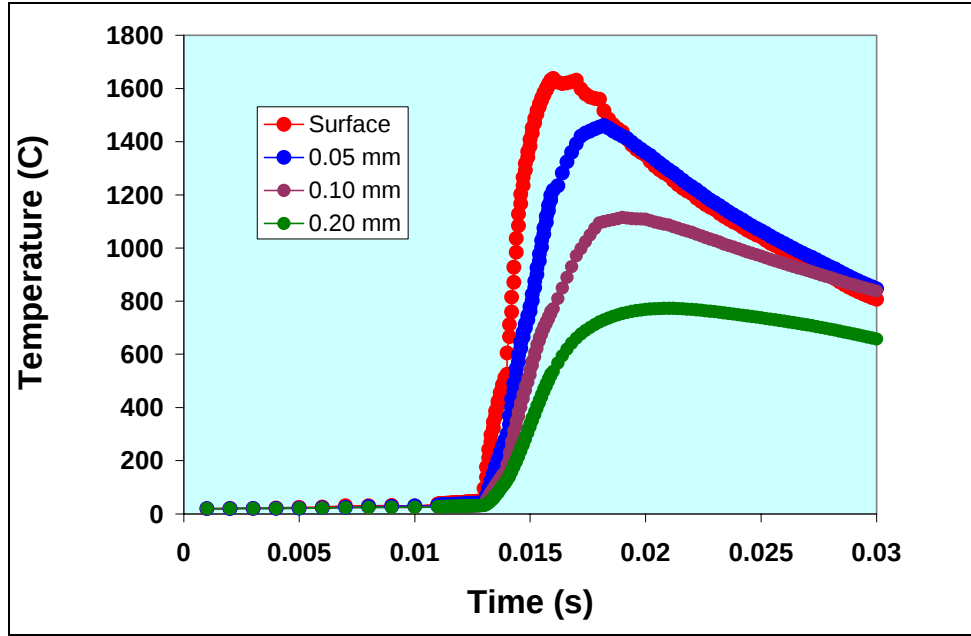
Figure 15. Temperature gradient from the surface in depth for the steel nozzle.
