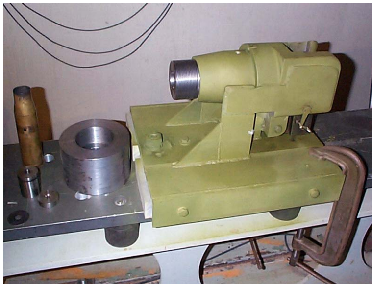
Figure 1. ARL 37-mm erosion fixture.
