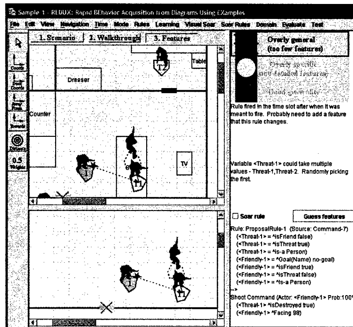
Figure 8. Immediate Detection of Errors
