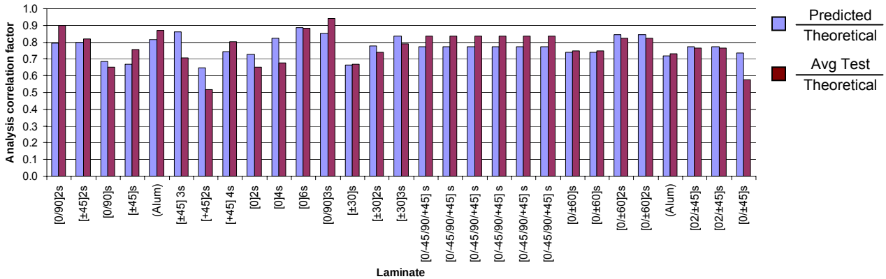
Fig. 5.6, Rolled up summary bar chart itemized by test specimen groups comparing \gamma_\mu from Table 5.7. Many different layup combinations tested. The blue bars represent the ratio of HyperSizer predicted buckling load over theoretical, where \gamma_\mu is computed with Equation (5.3.4). The dark red bars represent the ratio of average test buckling load over theoretical. These are test values that are found in the \gamma_\mu column of Tables 5.2 and 5.5. Included with the newly defined CF data are the calculated NASA knockdown factors and their resulting reliabilities. The average of these 109 individually backed out reliabilities is 99.04%, which gives independent verification to NASA's larger collection of test data and the intended buckling knockdown safety of 99%.
