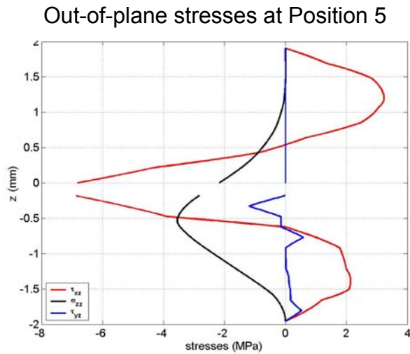
Fig. 6.10.11, Through-the-thickness distribution of interlaminar stresses at positions 5, as shown in Fig. 6.10.5
