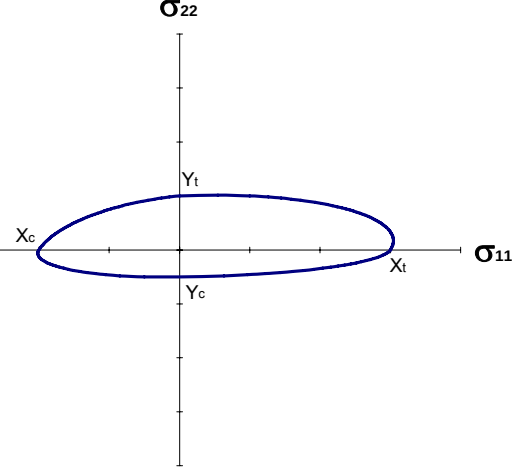
Fig. 7.5.4, Tsai-Hill with different compression/tension allowables
