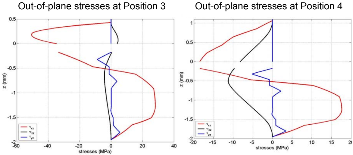
Fig. 6.10.9, Through-the-thickness distribution of interlaminar stresses at positions 3 and 4, as shown in Fig. 6.10.5
