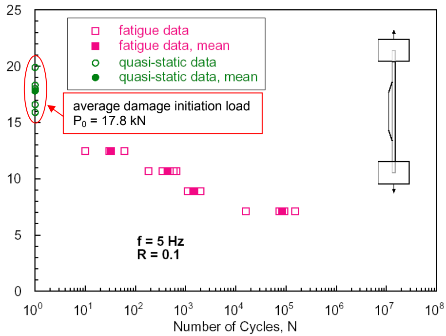
Fig. 6.10.6, Quasi-static and fatigue failure loads for the NASA tested skin/flange specimens. HyperSizer-BondJo results were compared only to the quasi-static data.
