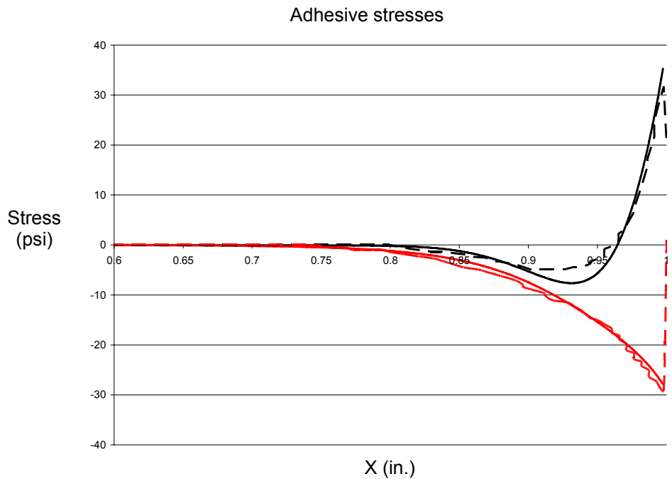
Fig. 6.9.8, Adhesive stress validation results between HyperSizer-BondJo and Stresscheck for panel applied moment.
