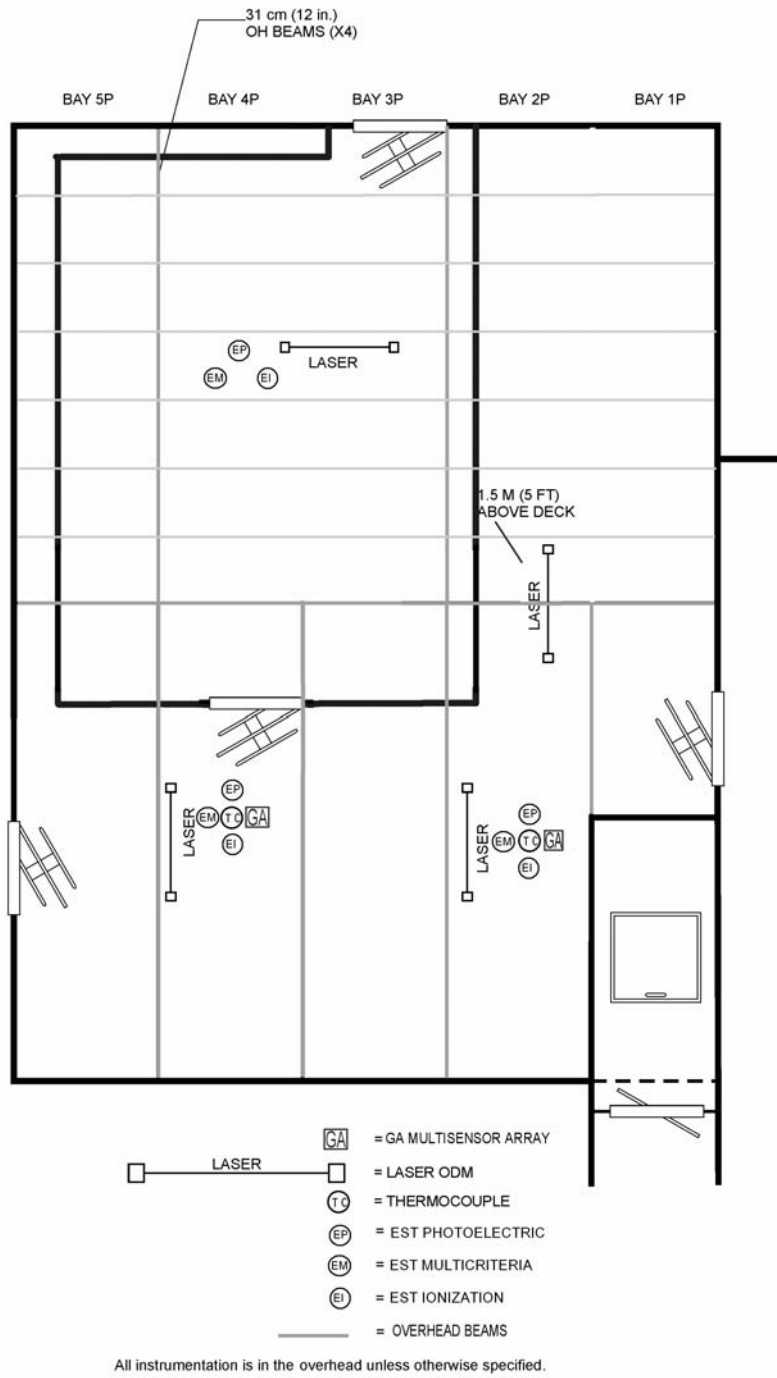
Fig. 10 — Layout of the GA sensor arrays, ODMs and smoke detectors in the 3 rd deck magazine
