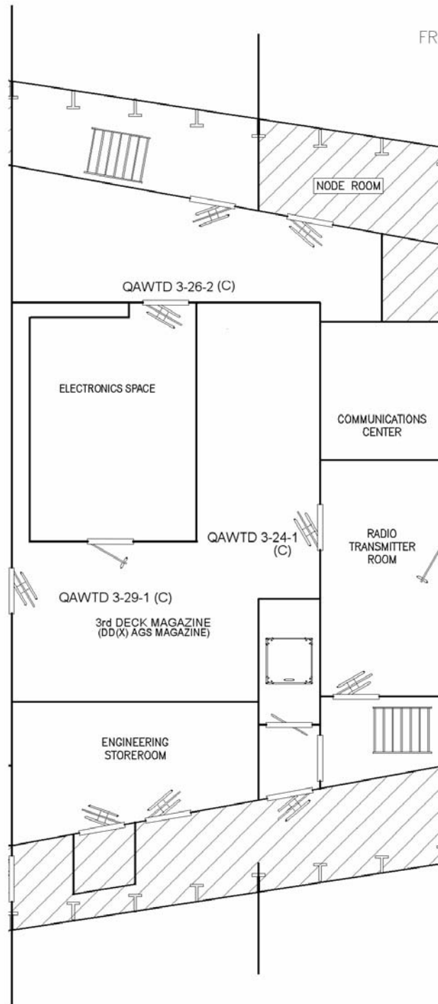
Fig. 1 — Layout of the spaces in the vicinity of the 3 rd deck magazine
