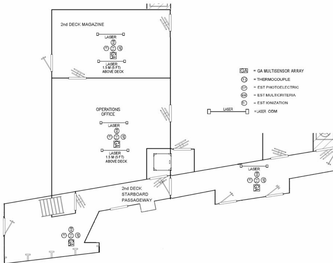
Fig. 12 — Locations of the GA sensor arrays, ODMs and spot-type detectors in 2 nd deck test compartments
