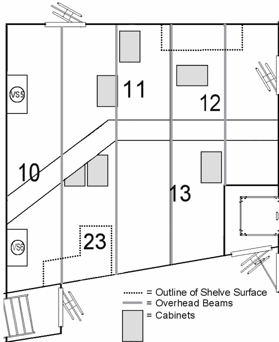
Fig. 5 — Layout of deck obstructions and source locations within 2 nd deck operations office
