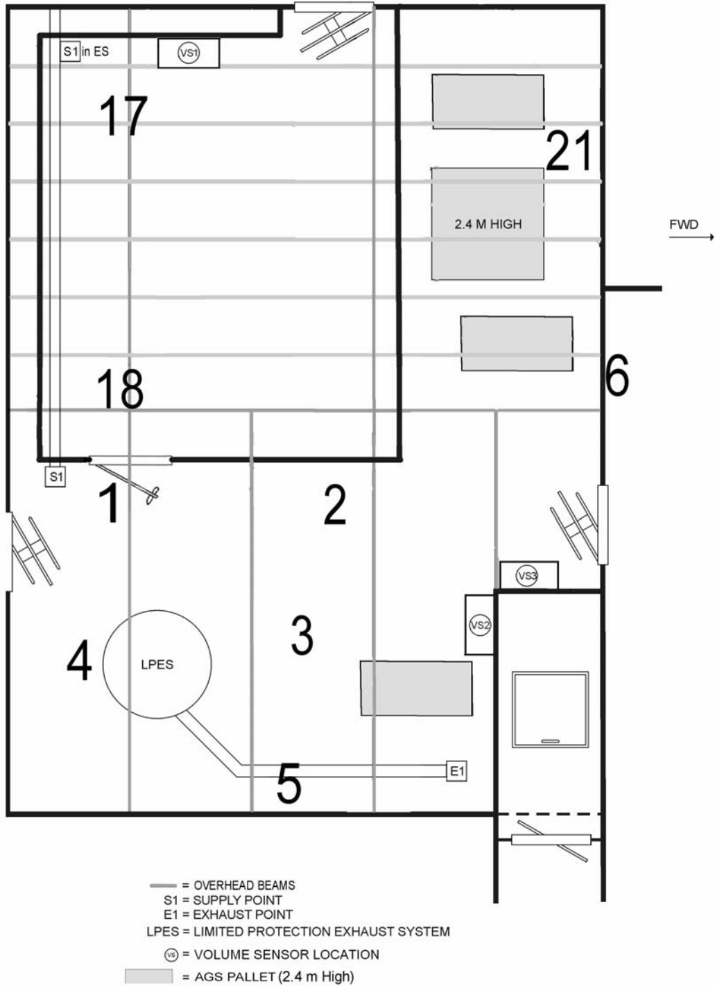
Fig. 3 — Layout of deck obstructions and source locations within 3 rd deck magazine
