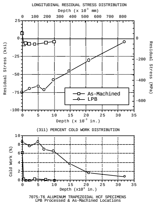
Figure 2 – Residual stress and cold work distributions produced by end milling and LPB in 7075-6.
