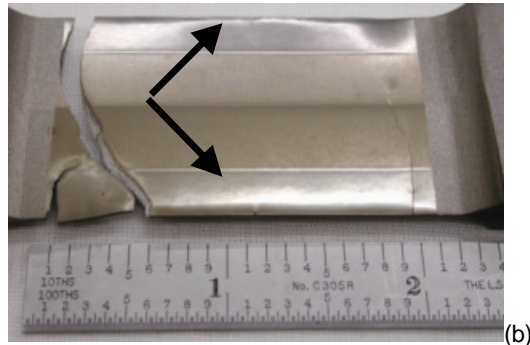
FIG. 10. (a) Optical fractograph of a SEB feature specimen with LPB treatment showing crack initiation from sub-surface regions (arrow). LPB + 0.5 mm (0.020 in.) FOD, R=0.1 , \sigma_{max}=690 MPa (100 ksi), N_f = 800,038 cycles, (b) Failure of a DEB feature specimen with LPB treatment showing initiation in a remote area in spite of the presence of 0.5 mm (0.020 in.) FOD (arrows) on both edges of the specimen. R=-1 , \sigma_{max} = 480 MPa (70 ksi), N_f = 174,315 cycles.
