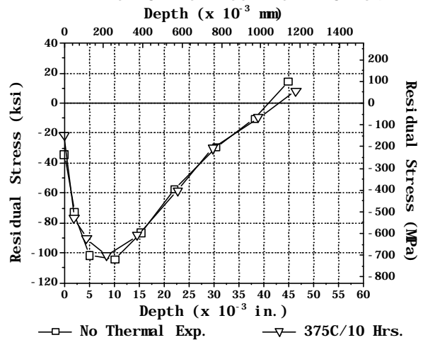
FIG. 14 – Residual stress distributions for LPB, showing a depth of compression over 0.04 in. and not significantly altered by thermal exposure to 375C for 10 hr.
