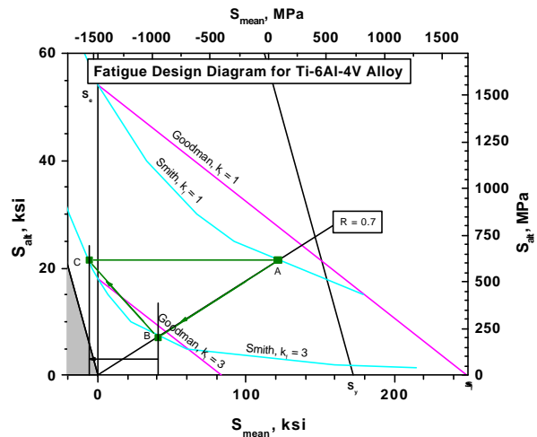
FIG 19. Section of the Fatigue Design Diagram illustrating the required magnitude of compression to fully mitigate the effect of FOD of k_f of 3.
