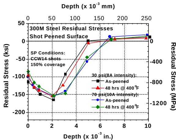
Figure 6 – SP subsurface residual stress distributions.
