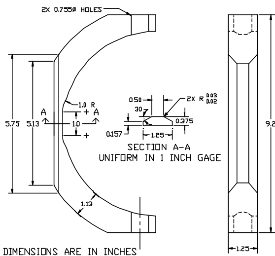
Figure 5 - C-ring specimen.
