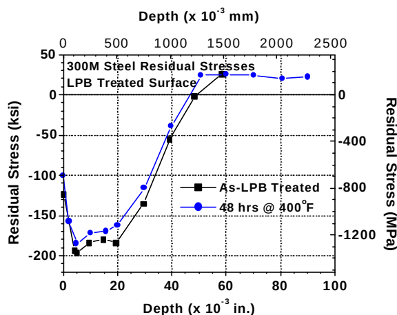
Figure 7 – LPB subsurface residual stress distributions.
