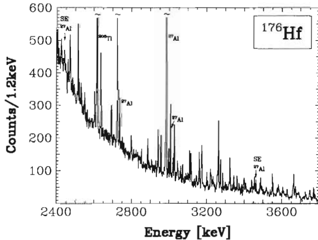
FIG. 2. Part of the ^{176}\text{Hf}(\gamma, \gamma') spectrum, measured at a scattering angle of 127^\circ using a bremsstrahlung beam of an end point energy of 4.1 MeV (linear ordinate scale). The selected extended section covers the energy range where the scissors mode strength is expected. Calibration lines ( ^{27}\text{Al} ) and background lines ( ^{208}\text{Tl} ) are marked (see text).
