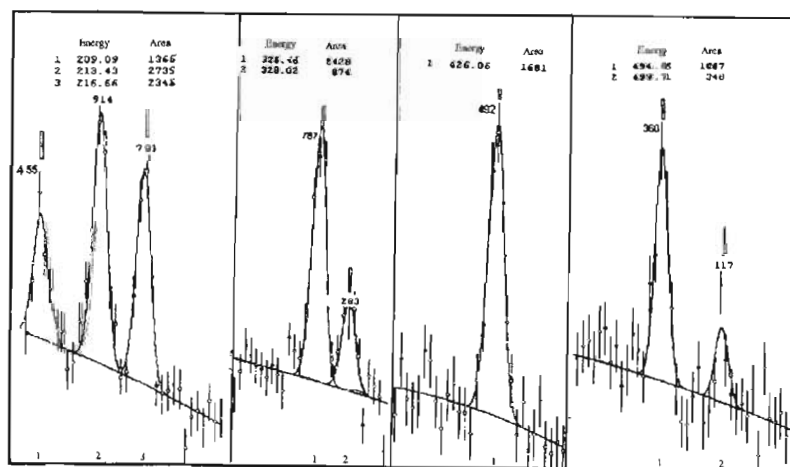
Fig. 2. Fragments of the \gamma spectrum obtained from the activated Ta sample. For each fragment, the observed lines are identified and their energies and areas are given as evaluated using the spectra-processing code. Six lines have energies that are in close agreement with the tabular values for ^{178\text{m}2}\text{Hf} : 213.4, 216.7, 325.6, 426.4, 495.0 and 574.2 keV (not shown).
