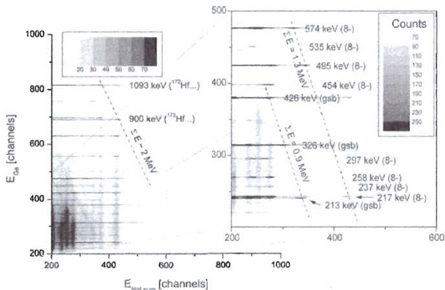
Figure 11. Contour plot of data taken with the miniball showing background radiation from the ^{178}\text{Hf}^{\text{m}2}/^{172}\text{Hf} sample. The zoom concentrates on gamma rays detected from ^{178}\text{Hf}^{\text{m}2} spontaneous decay. No bremsstrahlung was incident on the sample during acquisition of this data which was recorded for 11.5 h.
