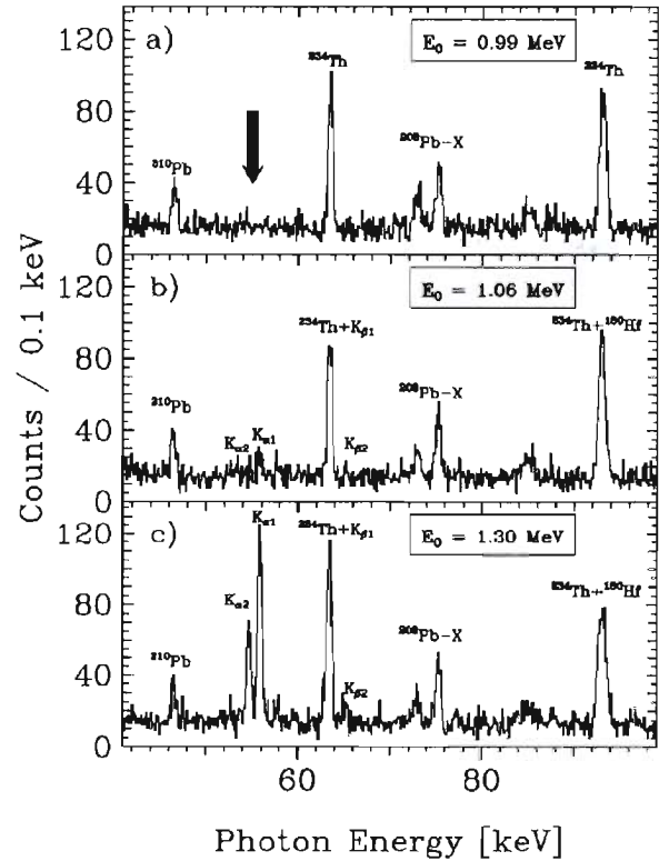
FIG. 2. Low-energy \gamma -ray and x-ray spectra of the enriched Ta sample from photoactivation at E_0=0.99 , 1.06, and 1.30 MeV (a), (b), and (c). The Hf characteristic x rays are labeled by K_{\alpha 1,2} and K_{\beta 1,2} . Background lines stemming from nuclear \gamma transitions in isotopes of natural decay chains or characteristic x rays are marked by the corresponding isotope symbols. In the top panel the energetic position of the Hf K_{\alpha} lines is indicated by a bold arrow.
