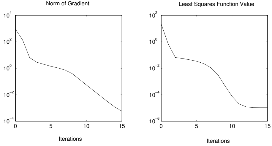
Figure 49: Levenberg-Marquardt for the seven parameter estimation problem
