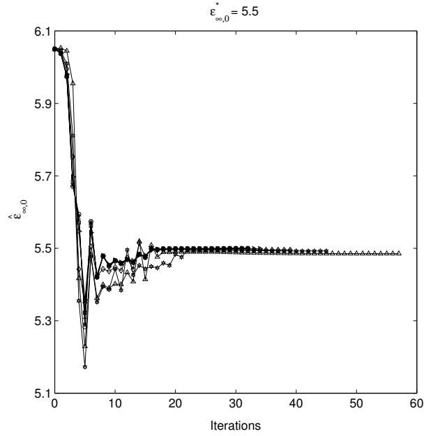
Figure 71: Levenberg-Marquardt for the three parameter estimation problem with added constant variance noise. Variation of the estimate \hat{\epsilon}_{\infty,0} with the iteration count.
