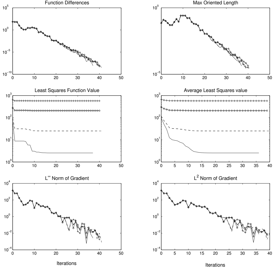
Figure 28: Nelder-Mead for the estimation of \epsilon_{s,0} and \kappa_s for water. The other five parameters are fixed at the values given in (103) and relative noise of varying levels is added to the data. 0% (—), 1% (---) 3% (o-) and 5% (+-)
