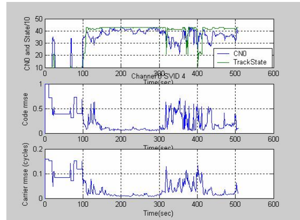
Figure 12 Indoor GPS Tracking (21 dB-Hz threshold)
