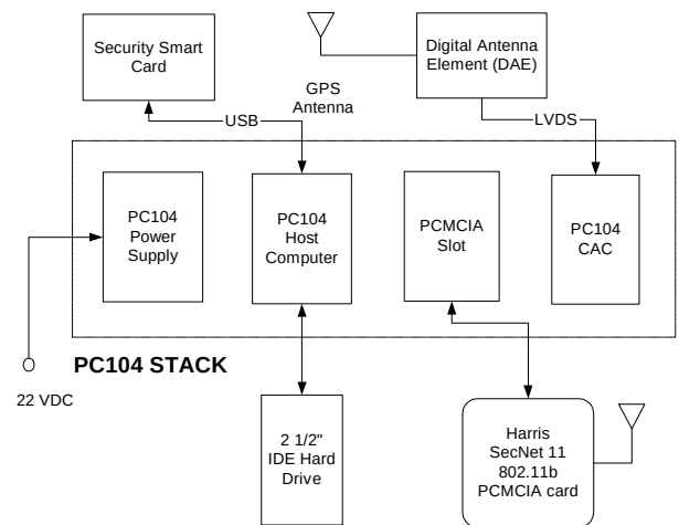
Figure 5 Software GPS Receiver Architecture
