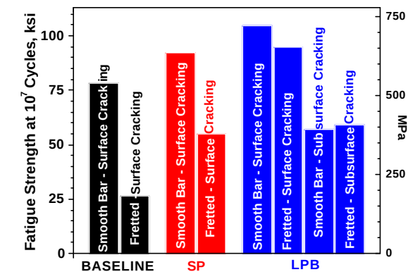
Figure 8 - Ti-6Al-4V fretting fatigue data for shot peened and LPB surface treatments.
