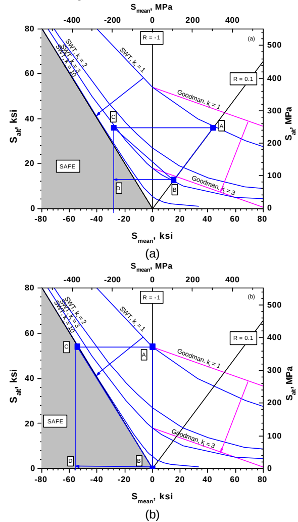
FIG. 6. Magnified sections of the fatigue design process with residual stresses in the presence of defects (FOD, pits or cracks). (a) Illustrates the effect of compressive stress (BD) to mitigate k_t = 3 for a fatigue condition of R=0.1 and in (b) the effect of compressive stress (BD) to mitigate a k_t = 1 is shown.
