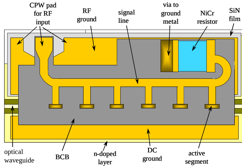
Figure 7. Schematic layout of the Segmented Traveling Wave EA modulator.
