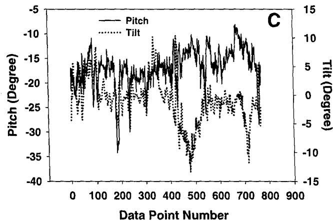
Figure D-1. Head position data from Flight 116, Pilot D's first flight, a low LOA slalom. The format used here is the same as used in Figure A-1.
