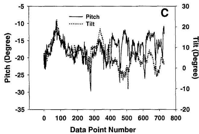
Figure B-4. Head position data from Flight 50, Pilot B's fourth flight, a low LOA slalom. The format used here is the same as used in Figure A-1.
