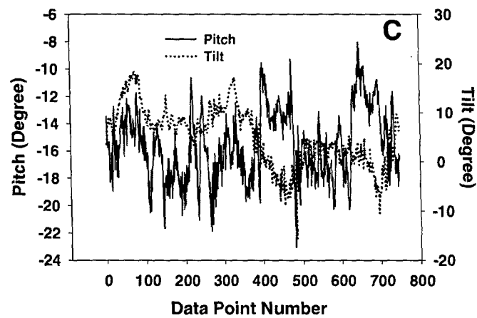
Figure B-1. Head position data from Flight 47, Pilot B's first flight, a low LOA slalom. The format used here is the same as used in Figure A-1.
