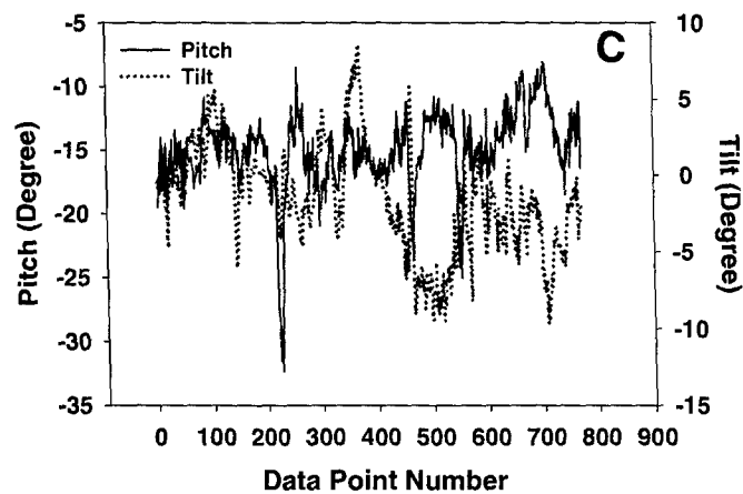
Figure D-3. Head position data from Flight 118, Pilot D's third flight, a low LOA slalom. The format used here is the same as used in Figure A-1.
