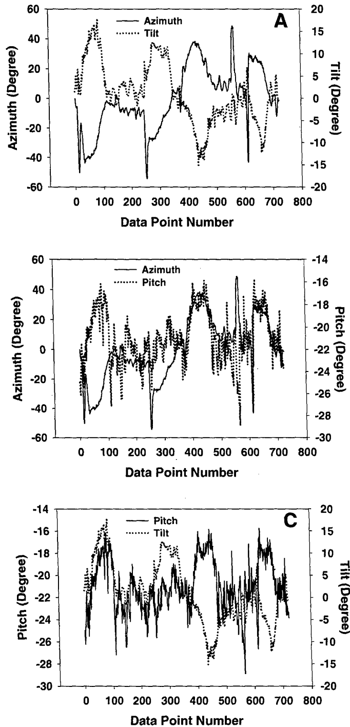
Figure A-1. Head position data from Flight 75, Pilot A's first flight, a low LOA slalom. The left axis of A shows head azimuth as the solid line while the right axis is head tilt as the dotted line; the left axis of B is head azimuth as the solid line while the right axis is head pitch as the dotted line; the left axis of C is head pitch as the solid line while the right axis is head tilt as the dotted line all in degrees and all as a function of time (10 data points = 1 second).
