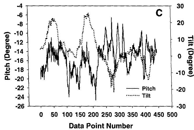
Figure B-5. Head position data from Flight 54, Pilot B's fifth flight, a moderate LOA slalom. The format used here is the same as used in Figure A-1.
