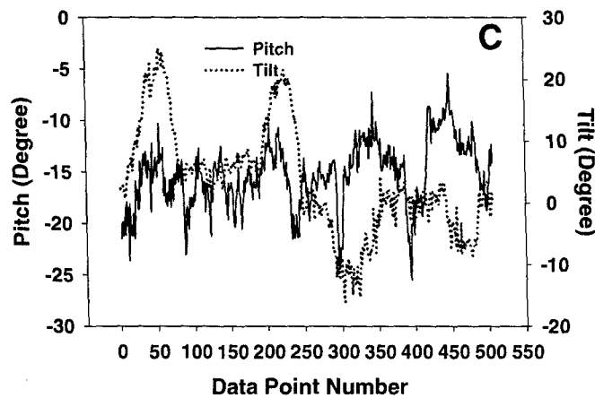
Figure B-9. Head position data from Flight 64, Pilot B's ninth flight, a moderate LOA slalom. The format used here is the same as used in Figure A-1.
