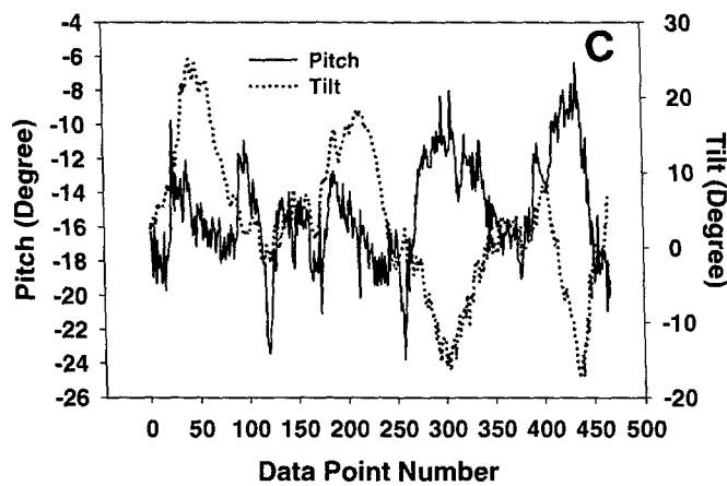
Figure B-11. Head position data from Flight 66, Pilot B's eleventh flight, a moderate LOA slalom. The format used here is the same as used in Figure A-1.
