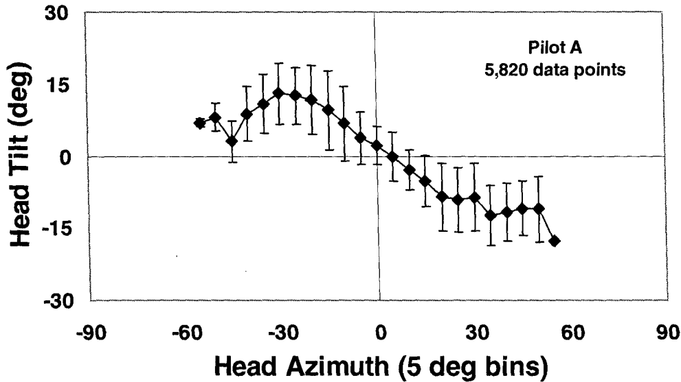
Figure 8. Head tilt average (with \pm 1.0 S.D.) as a function of head azimuth averaged across all Pilot A's eleven slaloms. Means and S.D. were calculated for the head tilts that were aggregated in azimuth bins of 5^\circ widths.
