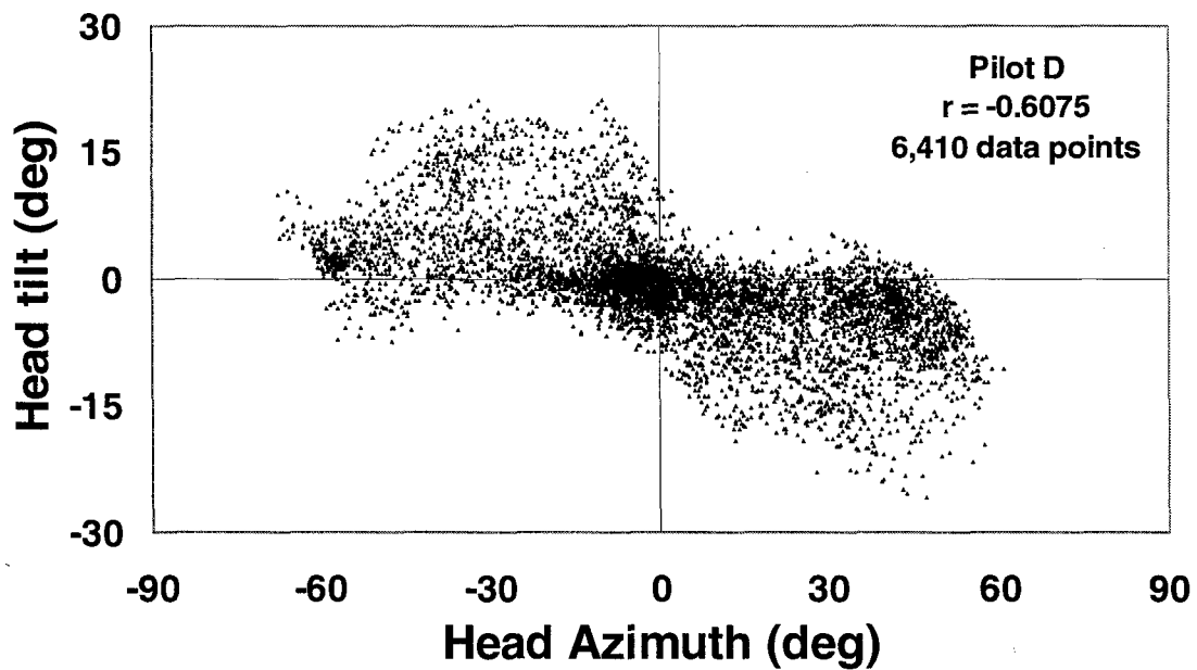
Figure 7. Scattergram of head tilt against head azimuth, both in degrees, for all Pilot D's slaloms.
