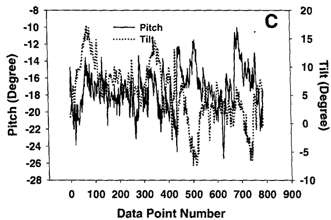
Figure B-3. Head position data from Flight 49, Pilot B's third flight, a low LOA slalom. The format used here is the same as used in Figure A-1.
