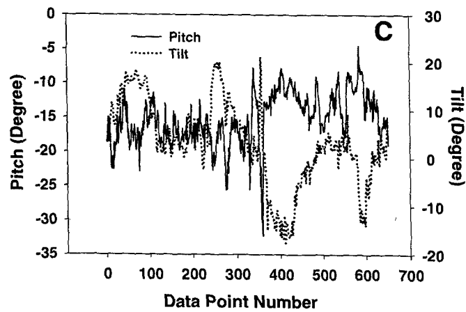
Figure C-2. Head position data from Flight 148, Pilot C's second flight, a low LOA slalom. The format used here is the same as used in Figure A-1.
