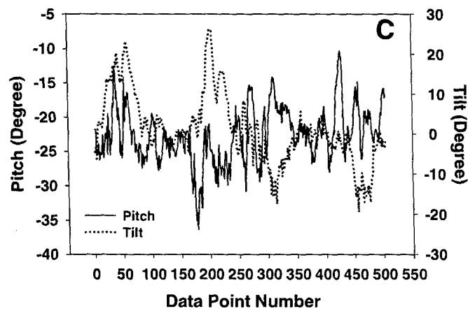
Figure C-8. Head position data from Flight 154, Pilot C's eighth flight, a moderate LOA slalom. The format used here is the same as used in Figure A-1.
