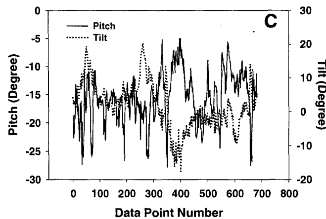
Figure C-1. Head position data from Flight 147, Pilot C's first flight, a low LOA slalom. The format used here is the same as used in Figure A-1.
