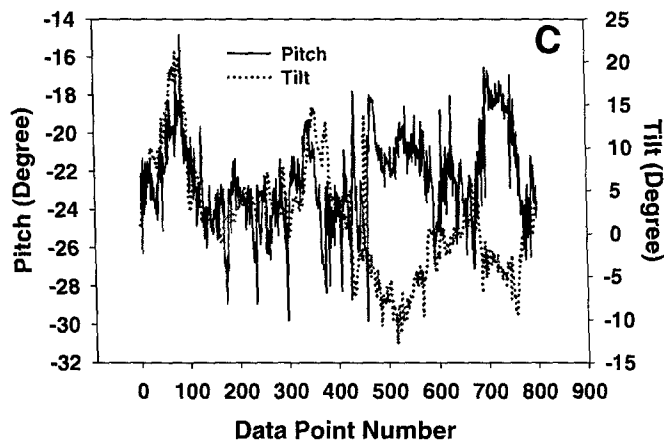
Figure A-3. Head position data from Flight 77, Pilot A's third flight, a low LOA slalom. The format used here is the same as used in Figure A-1.
