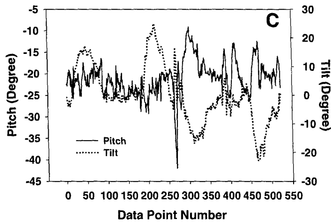
Figure C-6. Head position data from Flight 152, Pilot C's sixth flight, a moderate LOA slalom. The format used here is the same as used in Figure A-1.
