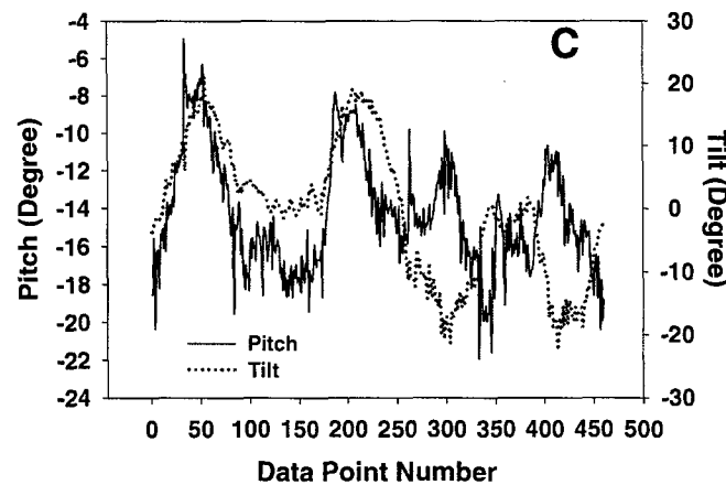
Figure A-6. Head position data from Flight 83, Pilot A's sixth flight, a moderate LOA slalom. The format used here is the same as used in Figure A-1.
