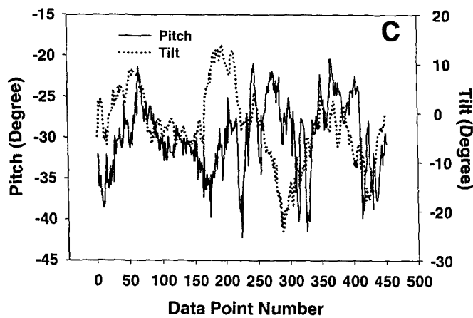
Figure D-5. Head position data from Flight 128, Pilot D's fifth flight, a moderate LOA slalom. The format used here is the same as used in Figure A-1.
