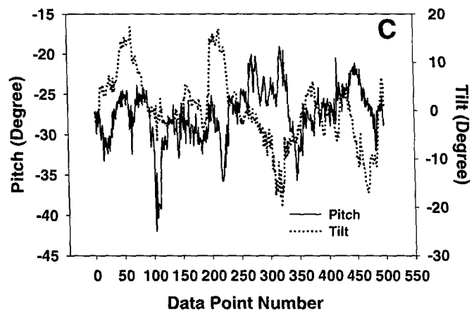
Figure D-9. Head position data from Flight 133, Pilot D's ninth flight, a moderate LOA slalom. The format used here is the same as used in Figure A-1.
