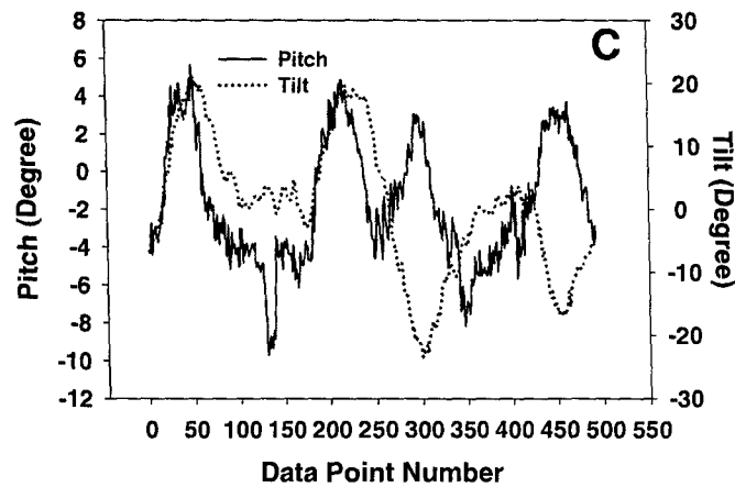
Figure A-11. Head position data from Flight 95, Pilot A's eleventh flight, a moderate LOA slalom. The format used here is the same as used in Figure A-1.
