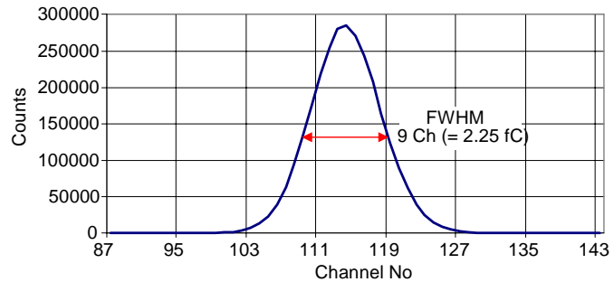
Figure 5. Histogram of signals from the analog electronics with a 44 fC test pulse input through a multiplexer.
