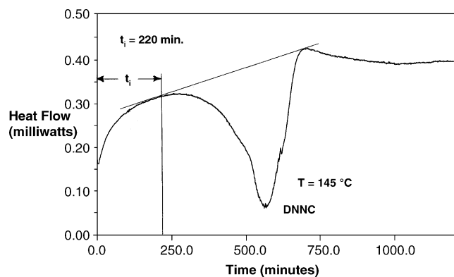
Fig. 4. Induction period ( t_i ) analysis for a DNNC run at 145 °C.
