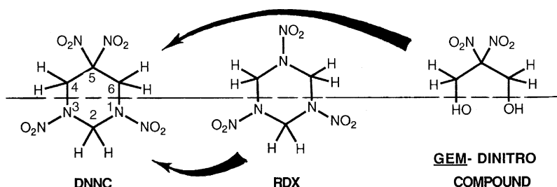
Fig. 1. Intramolecular hybrid structure of the DNNC molecule.
