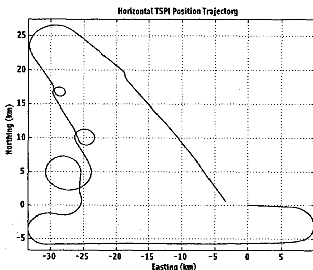
FIGURE 3. Horizontal TSPI Position Trajectory
