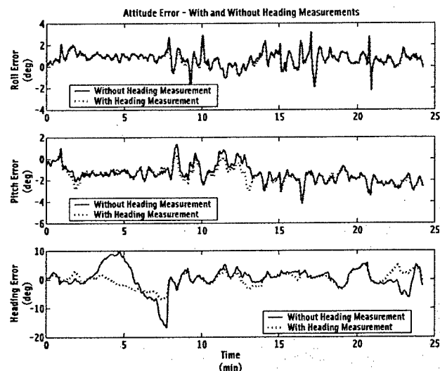
FIGURE 6. Attitude Error with and without GPS Heading Measurement
