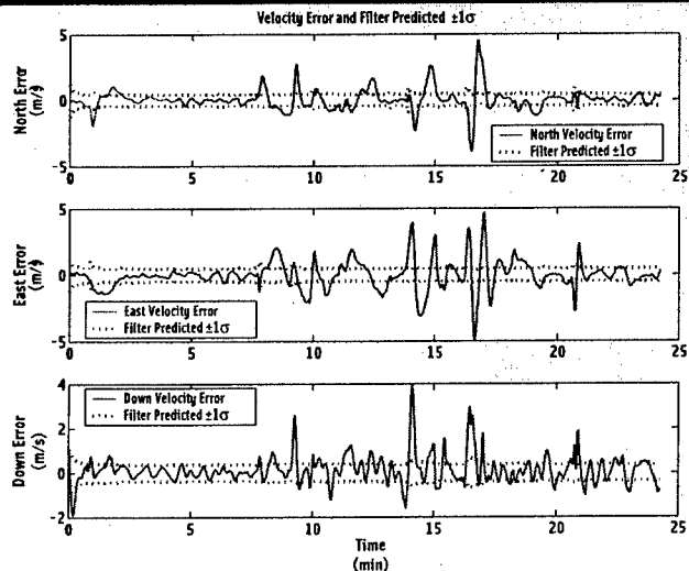
FIGURE 8. Velocity Error and Filter-Computed \pm 1\sigma Covariance
