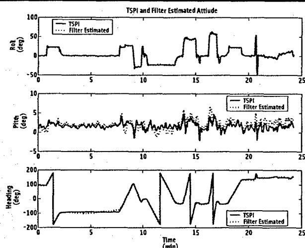
FIGURE 4. TSPI and Filter-Estimated Attitude
