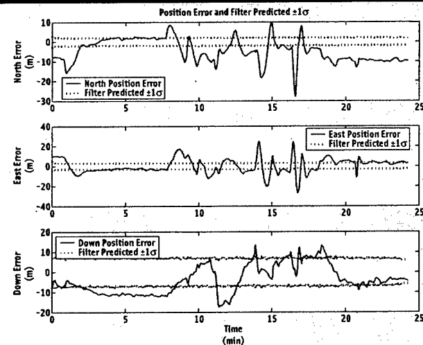
FIGURE 7. Position Error and Filter-Computed \pm 1\sigma Covariance
