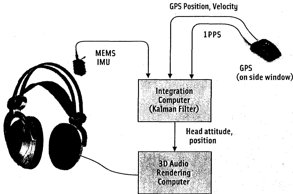
FIGURE 1. Head Tracker for 3D Audio System Configuration
