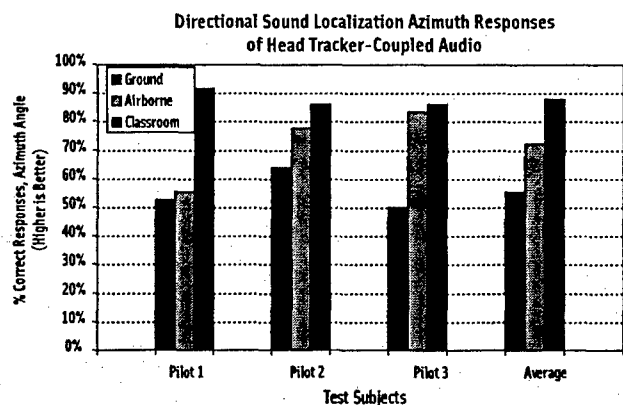
FIGURE 10. Head Tracker-Coupled Localization Azimuth Response Performance
