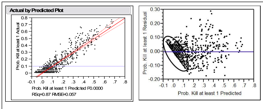
Figure 35. Actual vs. Predicted Probability to destroy at least one platform and Residual vs. Predicted Probability to destroy at least one platform.
