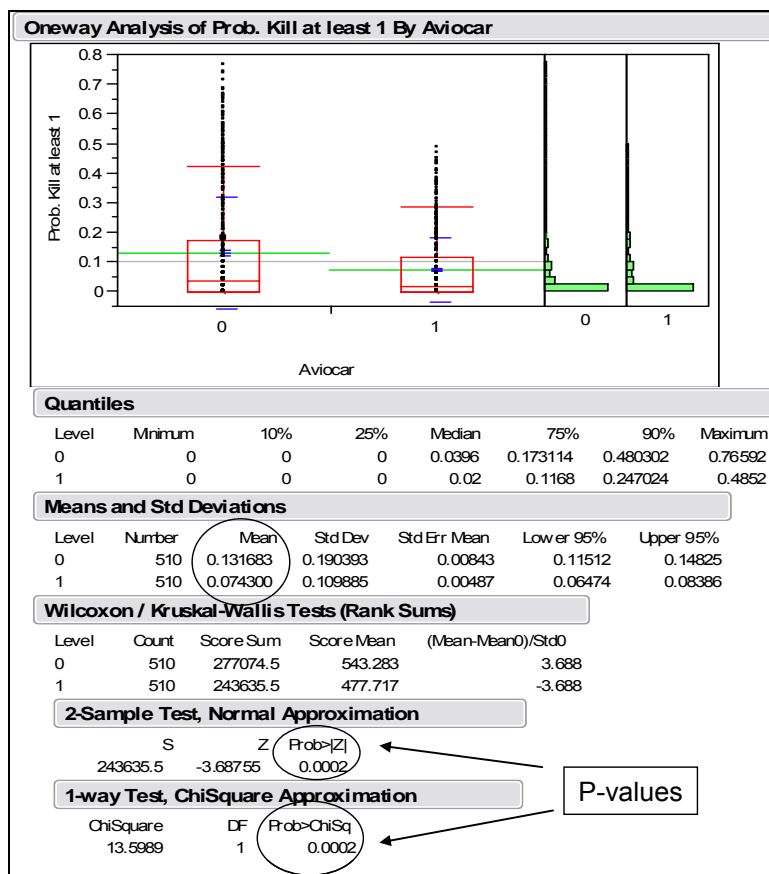
Figure 29. One-way analysis of means of the probability of destroying at least one platform with the AVIOCAR MPA in the model.
