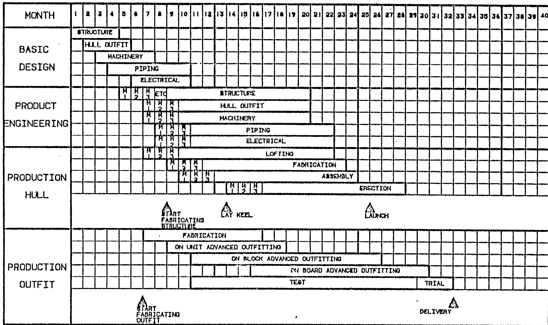
FIGURE 9 -ADVANCED SHIPBUILDING AND INTEGRATED ENGINEERING
