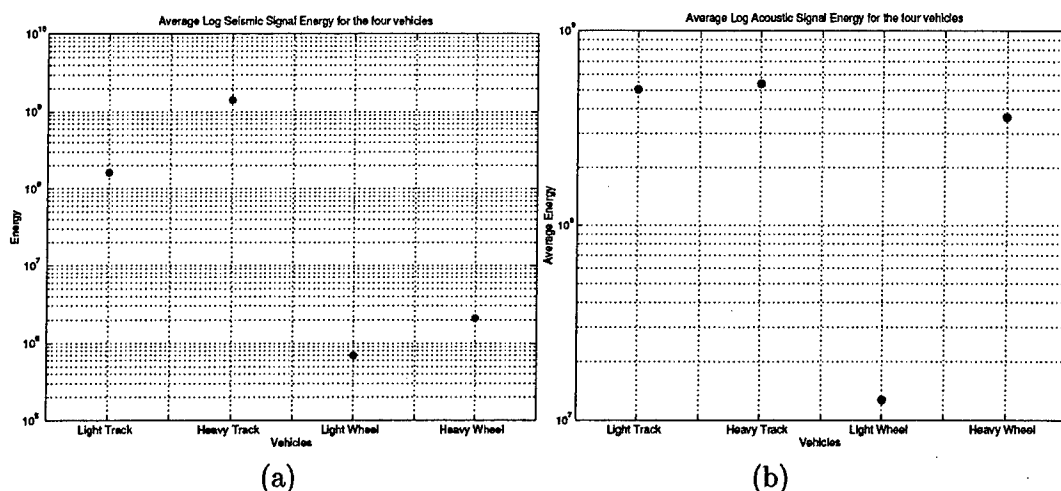
Figure 2.3: Average signal energy on a log scale for LT, HT, LW and HW vehicles: (a) seismic data, and (b) acoustic data. Each plot only has four data points, one for each class of vehicles.
