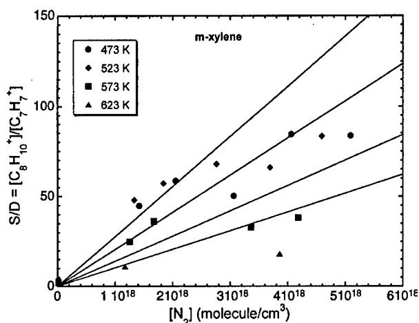
Fig. 2. TIFT measurements of S/D for the m -xylene cation as a function of number density of N_2 (50–250 Torr) over the temperature range 473–623 K. The lines for T=473, 523, 573 and 623 K (from top to bottom) show modeling results with -\langle\Delta E\rangle/hc = 280\text{ cm}^{-1} , see text.
