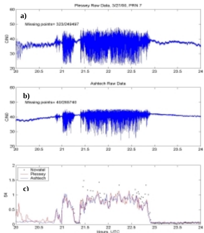
Figure 1. Data collected 27 March 2000 a) 10 Hz C/N 0 from the Plessey Receiver; b) 20 Hz C/N 0 from the Ashtech and c) Comparisons of S4 calculated over 60 sec intervals from the Plessey, Ashtech and ISM
