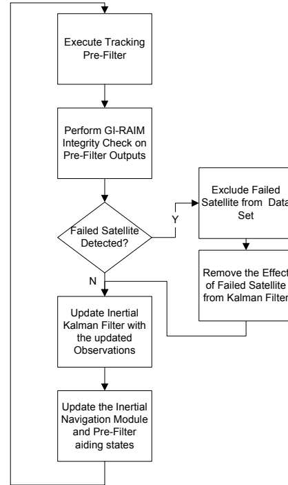
Figure 5 GI-RAIM Algorithm Steps
