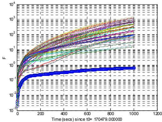
Figure 11 FDI Detection metric (F) of correct ambiguity
