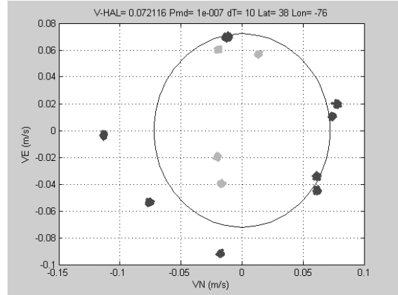
Figure 8 Velocity Horizontal Alarm Limits for HAL=1.3, VAL=2.0 and dT=10 (Grey marks undetected satellite failures, Black marks detected satellite failures)
