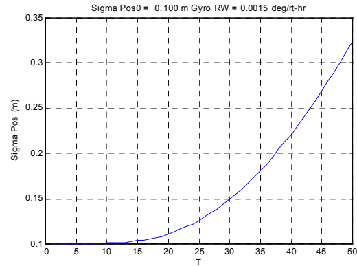
Figure 7 Inertial Position Error Propagation with No Initial Velocity Error
