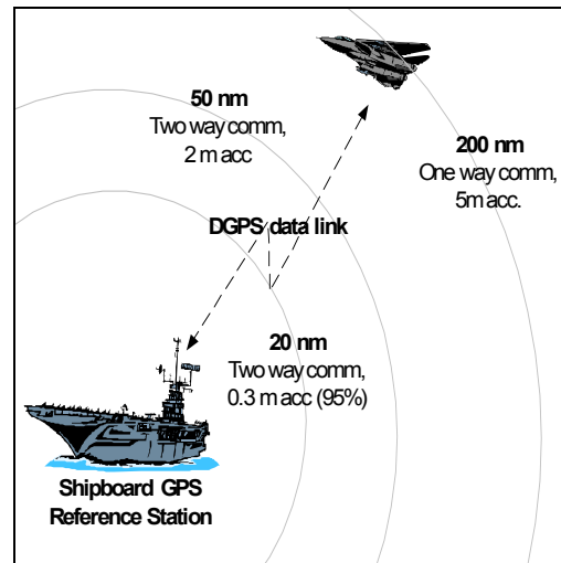
Figure 1 JPALS Shipboard Concept
