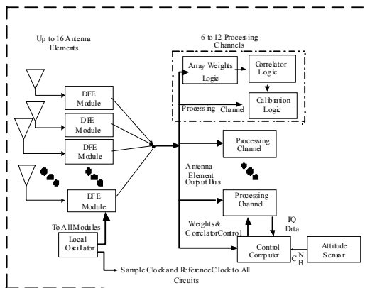
Figure 3 GPS Spatial Signal Processing
