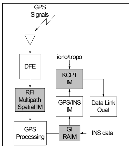
Figure 1 Integrity Monitoring Concept
