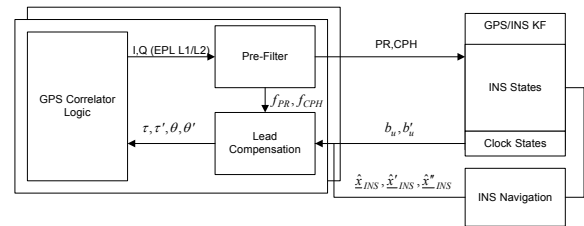
Figure 4 Cascaded GPS/Inertial Filter Approach
