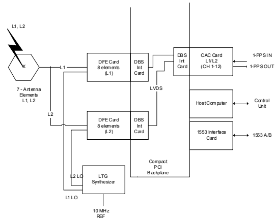
Figure 12 A 7-element L1/L2 HAGR-A Configuration
