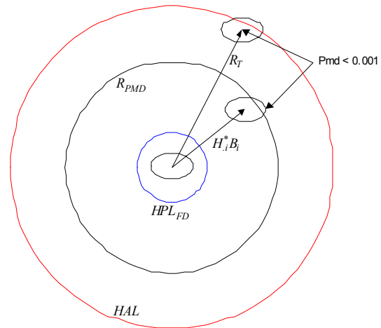
Figure 6 BPOD Principle of Operation
