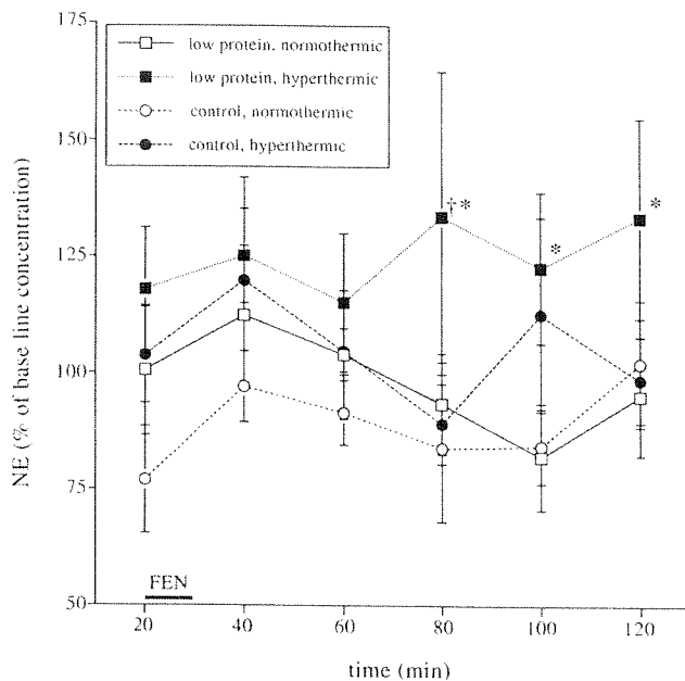
Fig. 3. Percentage of mean \pm S.E.M. baseline extracellular NE concentration in rat ventral striatum. Significant difference vs. low protein, normothermic rats ( p < 0.05 ). Significant difference vs. control, hyperthermic rats ( p < 0.05 ).
