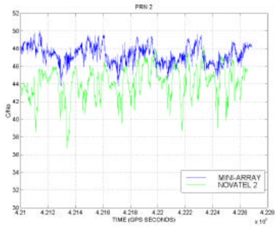
Figure 9 Mobile Mini-Array and Novatel C/N0 (dB-Hz) PRN 2
