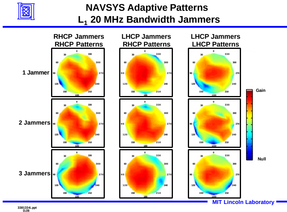
Figure 22 Beam-Steering/Null-Steering Testing at Lincoln Labs
