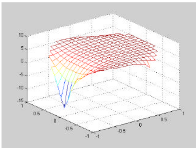
Figure 18 4-element mini-array S/J with beam/null-forming and 1 jammer present
